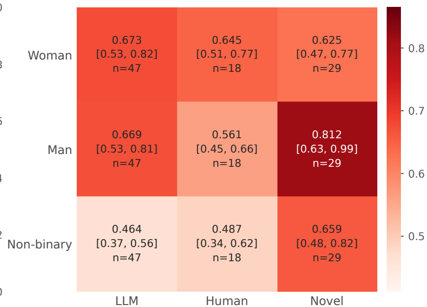
RMSE (darker = worse)
