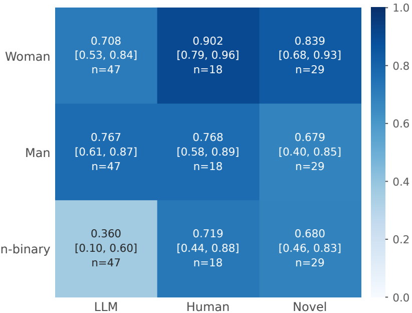
Pearson r (darker = better)
