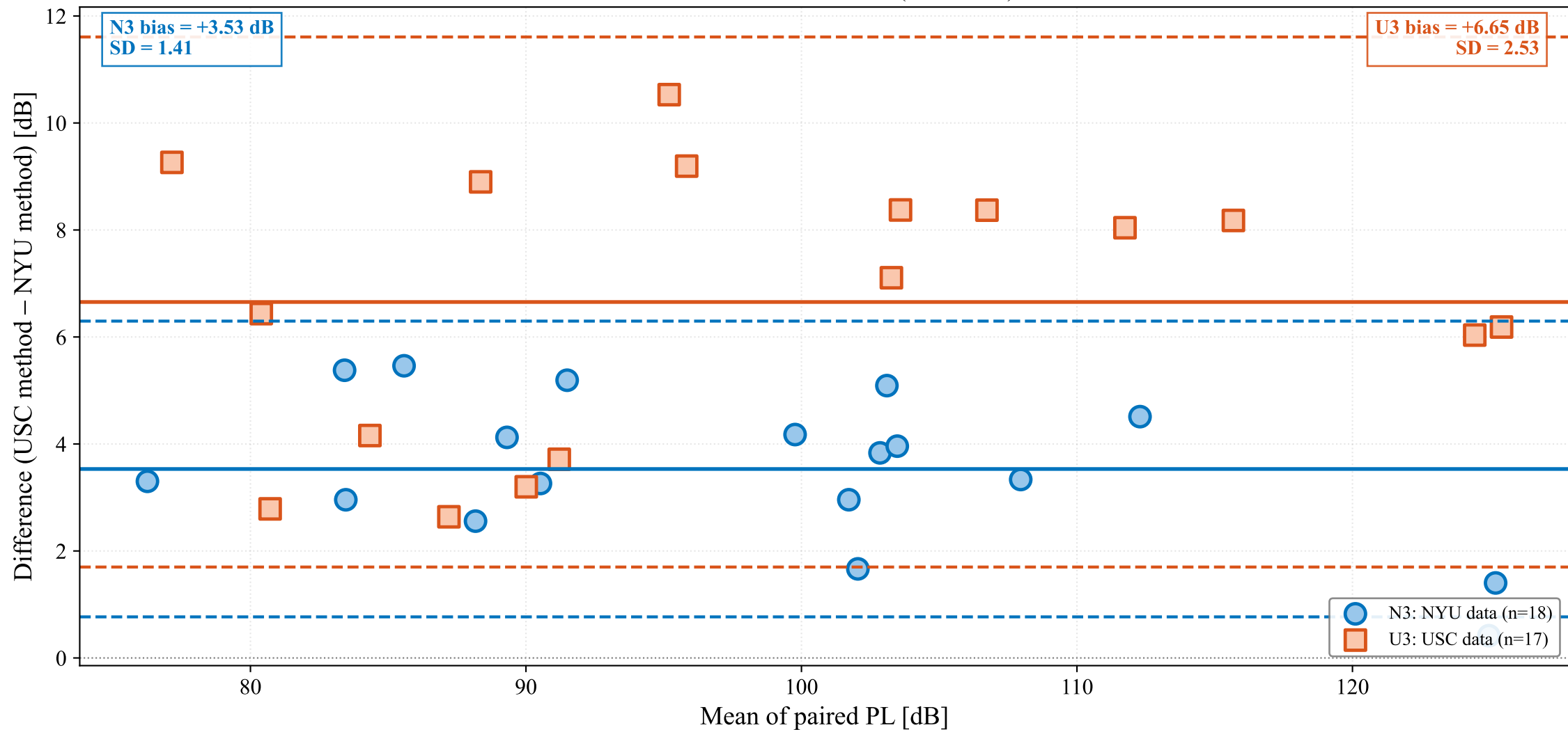
Bland-Altman: Omni PL (6.75 GHz)
