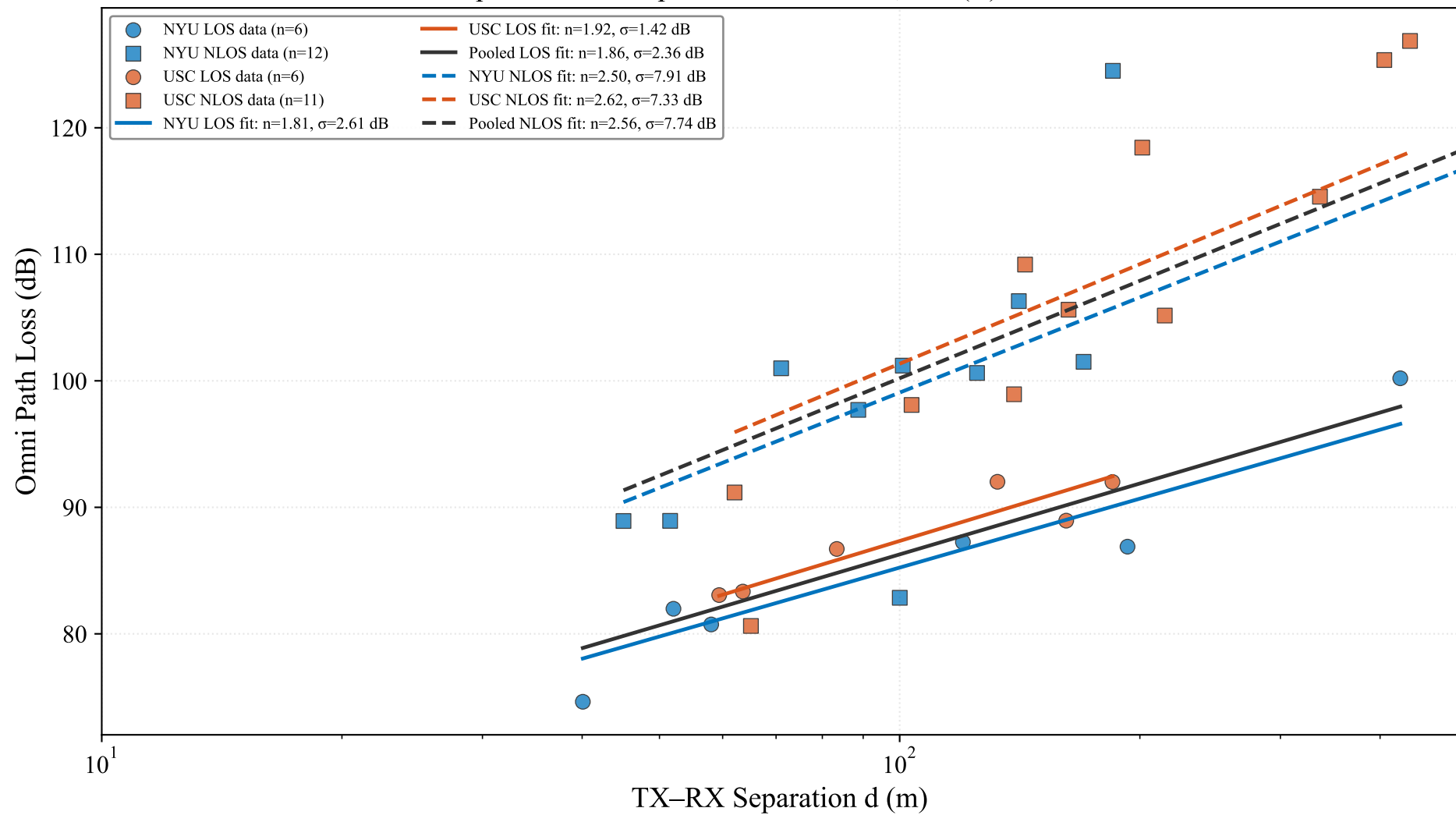
CI path-loss fit — pooled NYU + USC, FR1(C) 6.75 GHz
