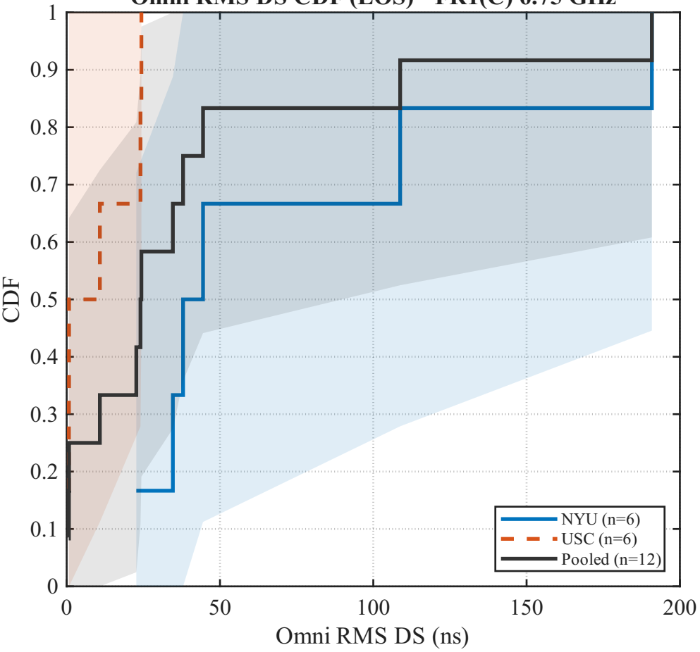
Omni RMS DS CDF (LOS) - FR1(C) 6.75 GHz
