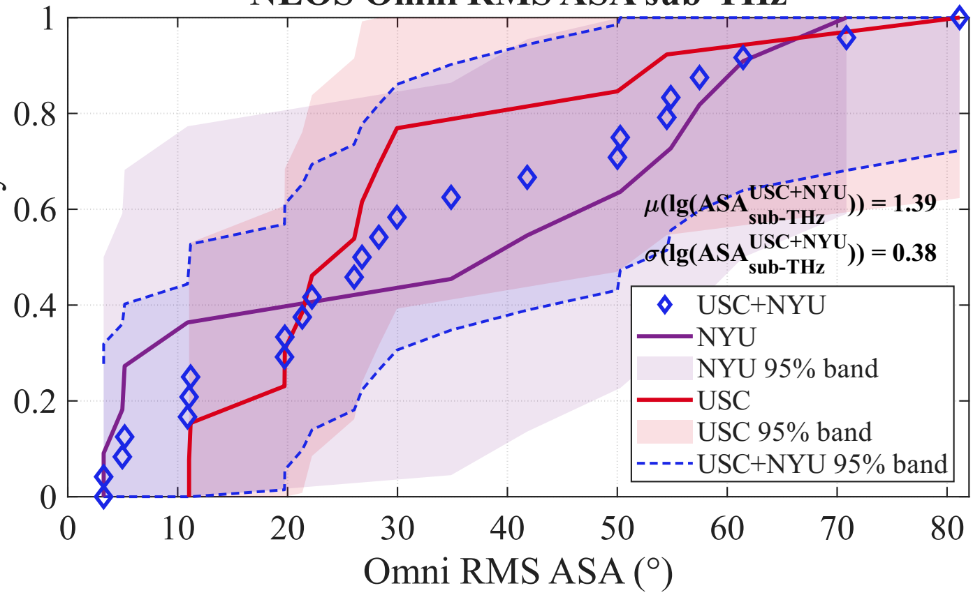
NLOS Omni RMS ASA sub-THz
