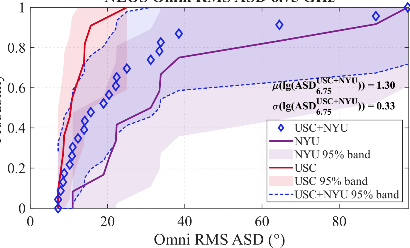
NLOS Omni RMS ASD 6.75 GHz
