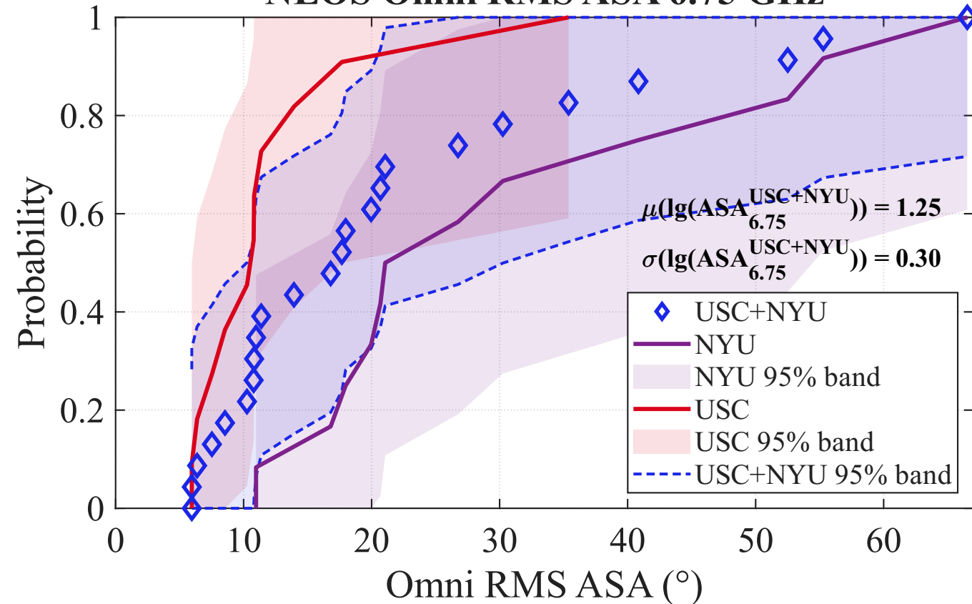
NLOS Omni RMS ASA 6.75 GHz
