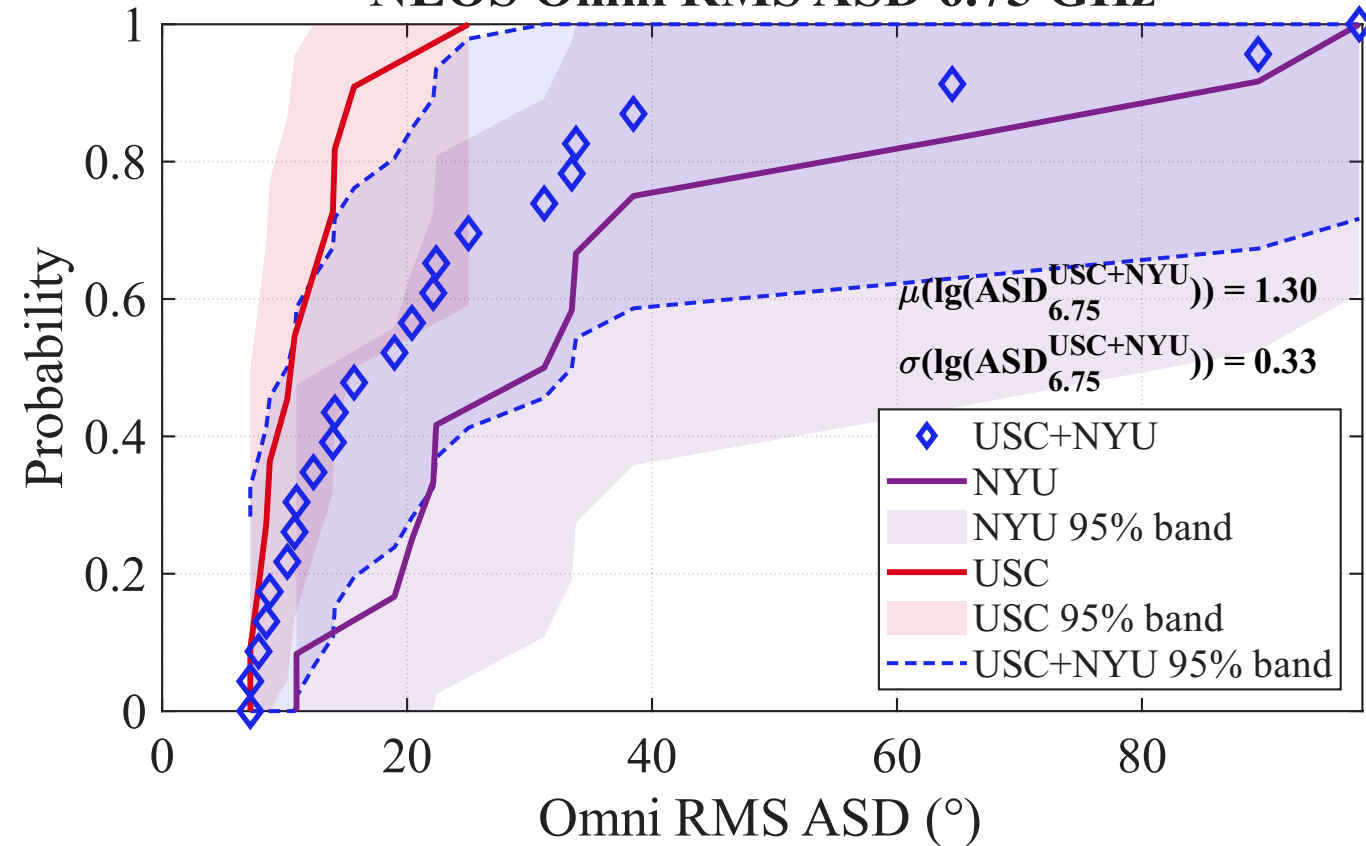
NLOS Omni RMS ASD 6.75 GHz
