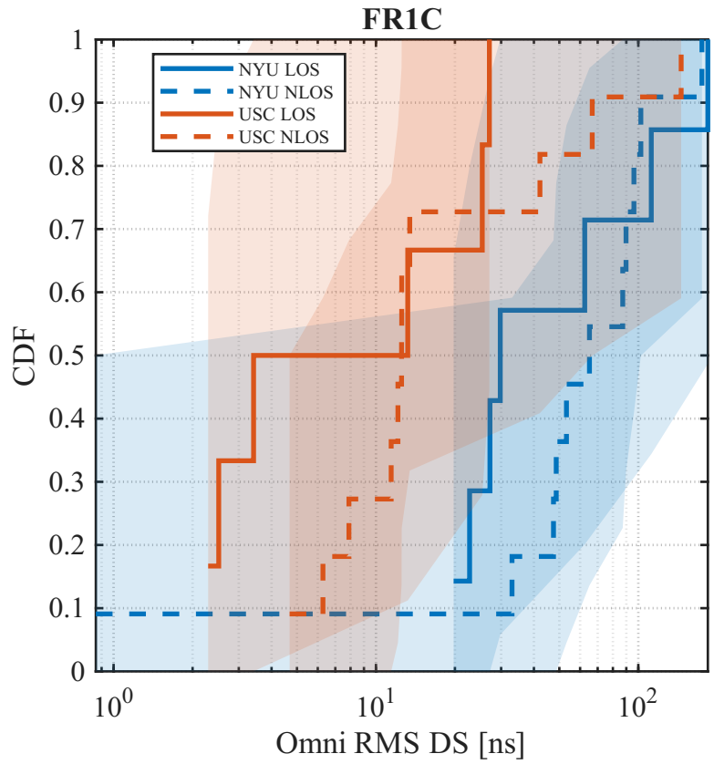
Omni RMS Delay Spread CDFs with DKW 95% bands
