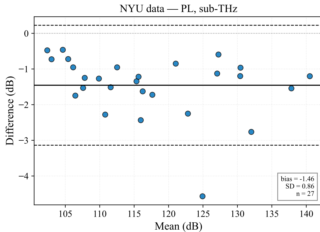
Fig. 3 — Bland-Altman: PL & Omni DS cross-processing (sub-THz)
