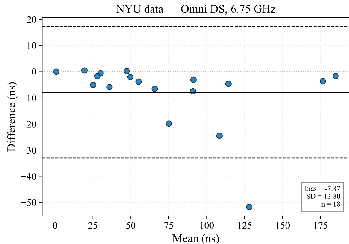
Fig. 3 — Bland-Altman: PL & Omni DS cross-processing (6.75 GHz)
