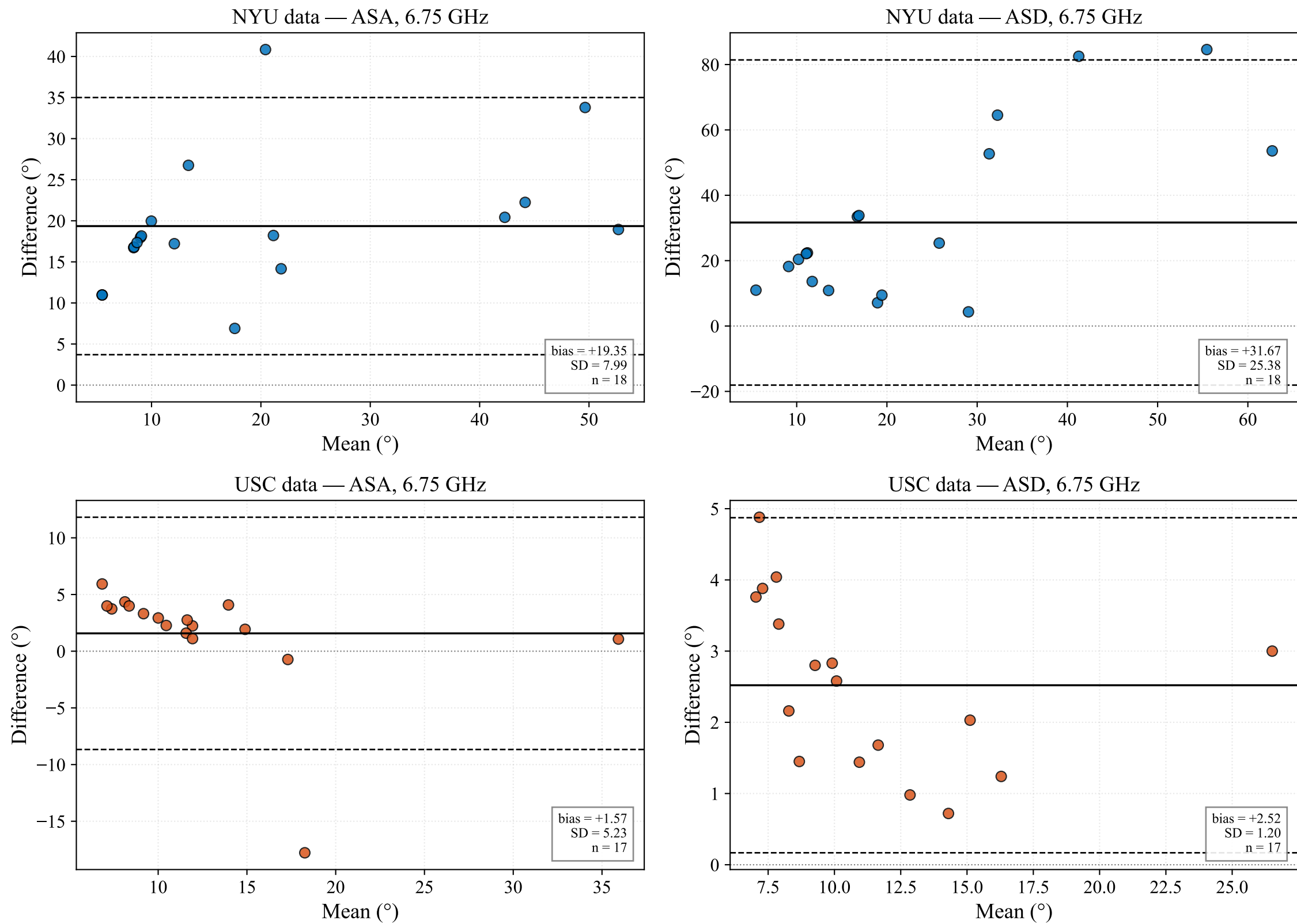
Fig. 4 — Bland-Altman: ASA & ASD cross-processing (6.75 GHz)
