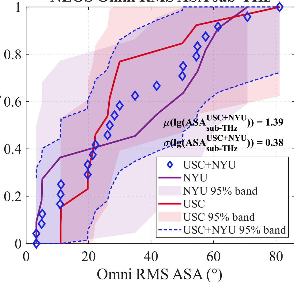
NLOS Omni RMS ASA sub-THz
