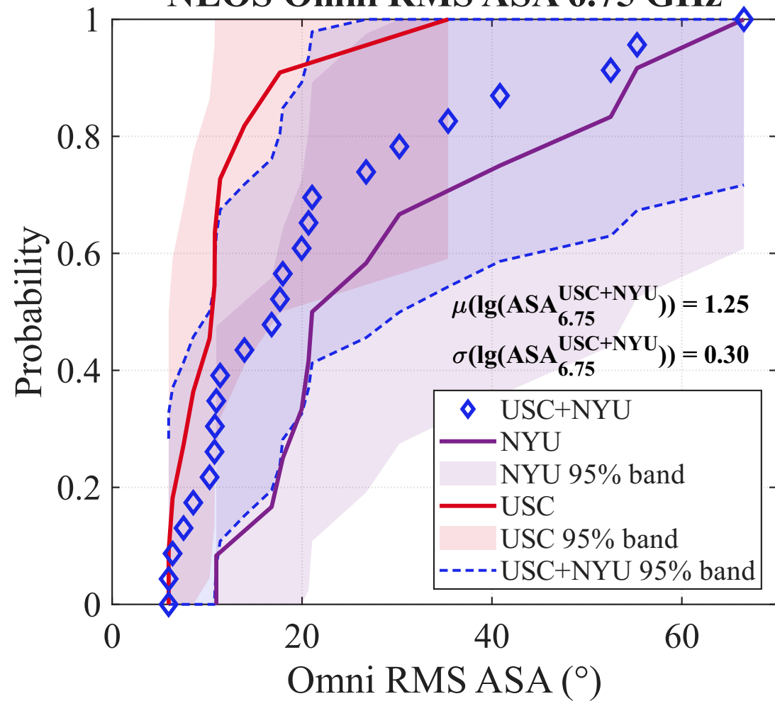
NLOS Omni RMS ASA 6.75 GHz
