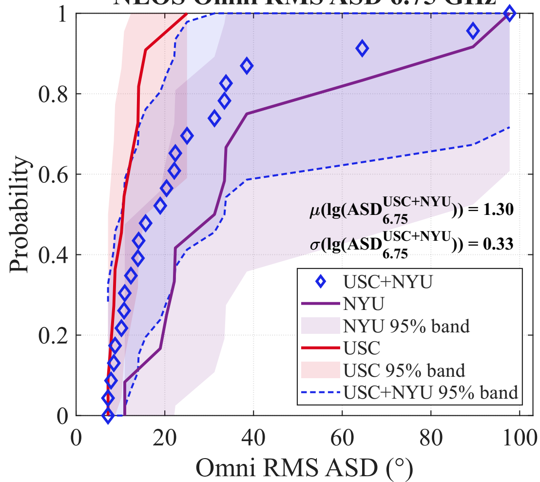
NLOS Omni RMS ASD 6.75 GHz
