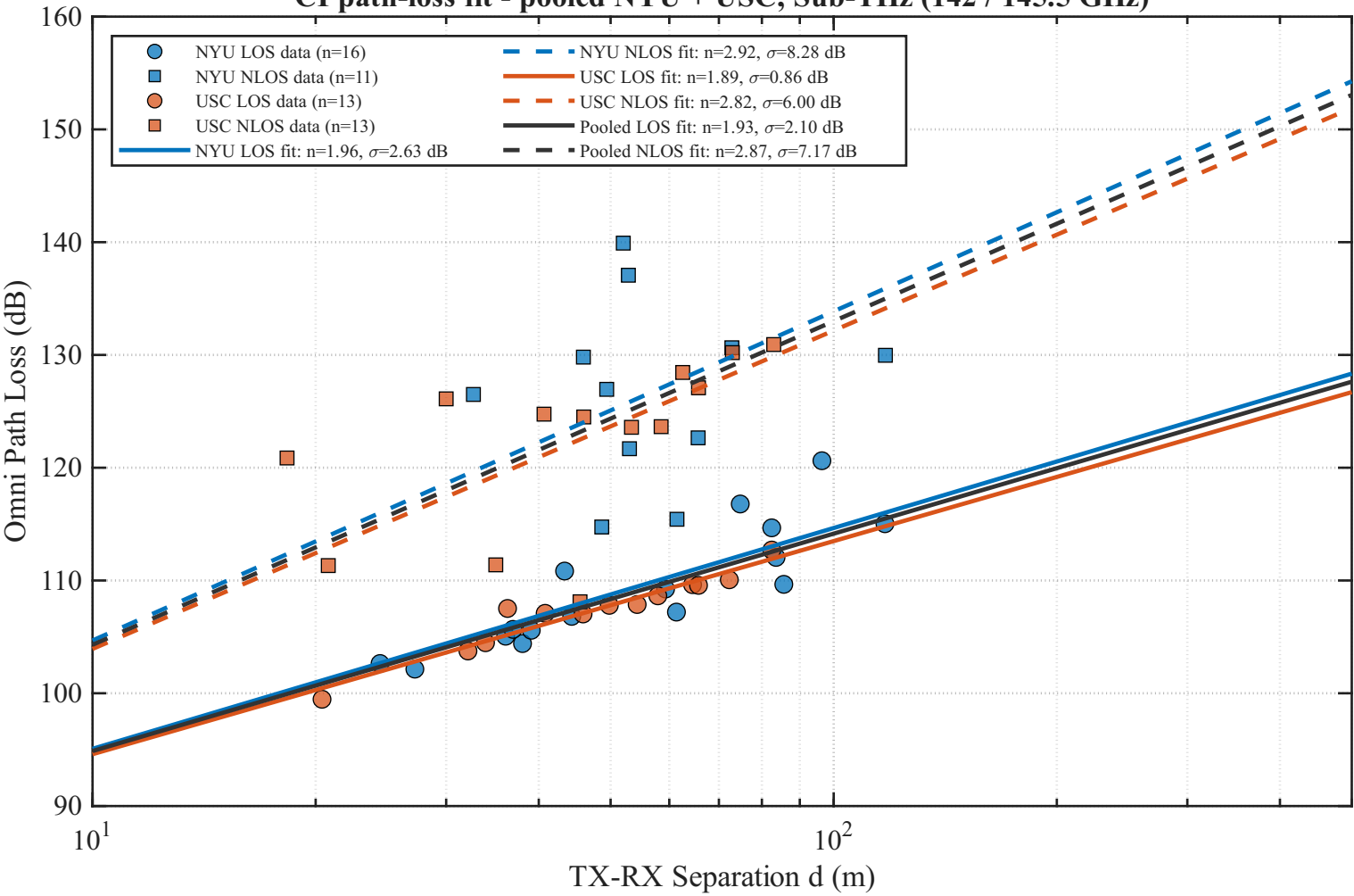
CI path-loss fit - pooled NYU + USC, Sub-THz (142 / 145.5 GHz)
