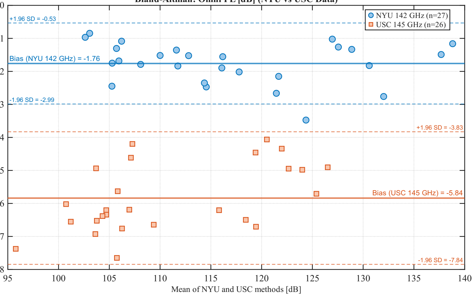
Bland-Altman: Omni PL [dB] (NYU vs USC Data)
