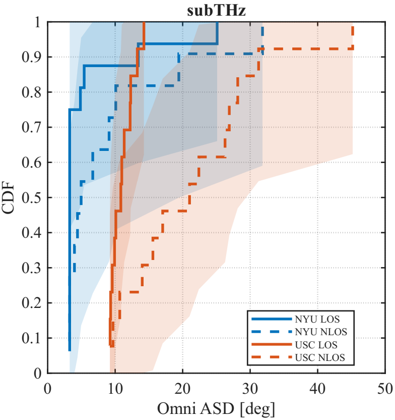
Omni ASD CDFs with DKW 95% bands
