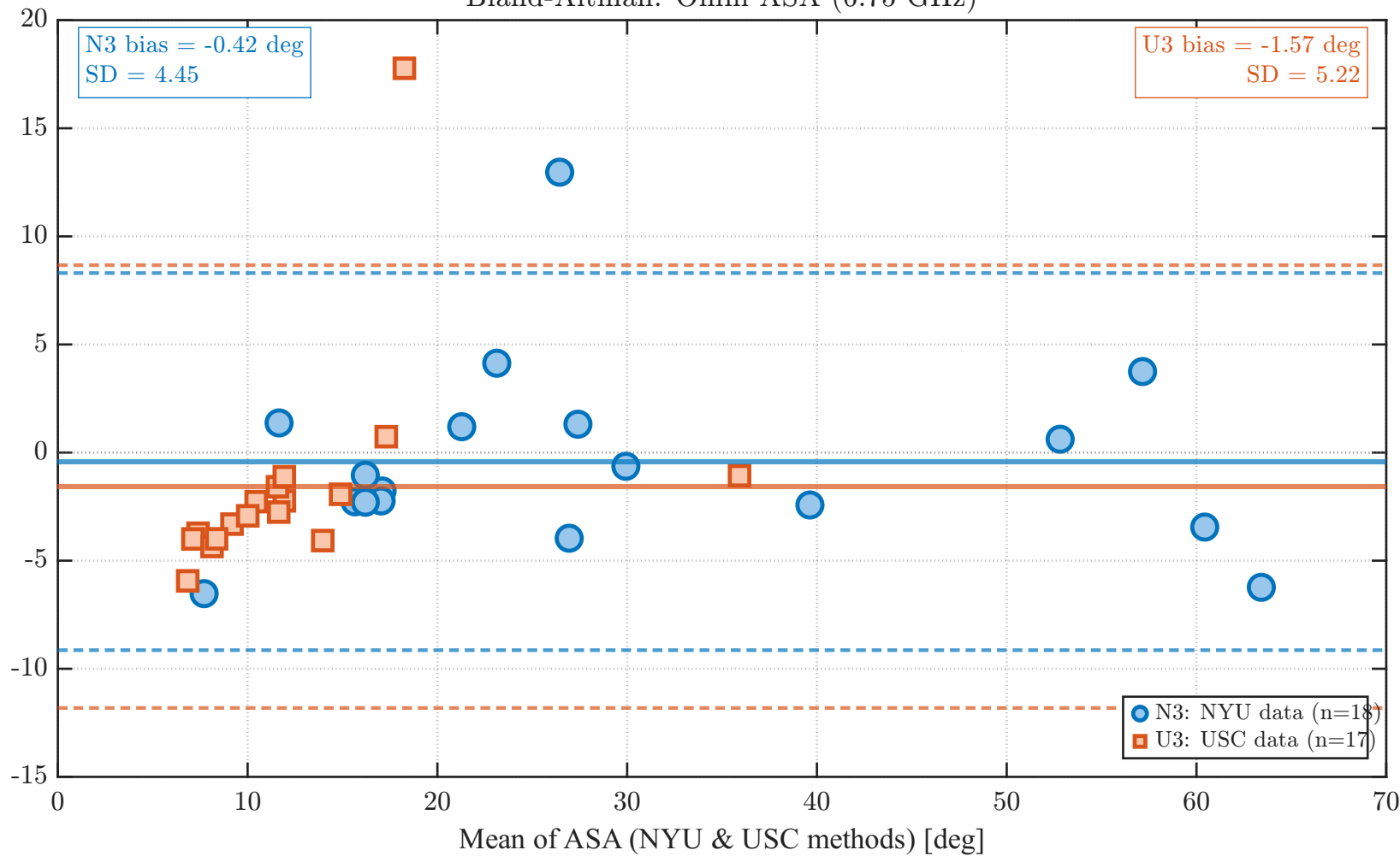
Bland-Altman: Omni ASA (6.75 GHz)
