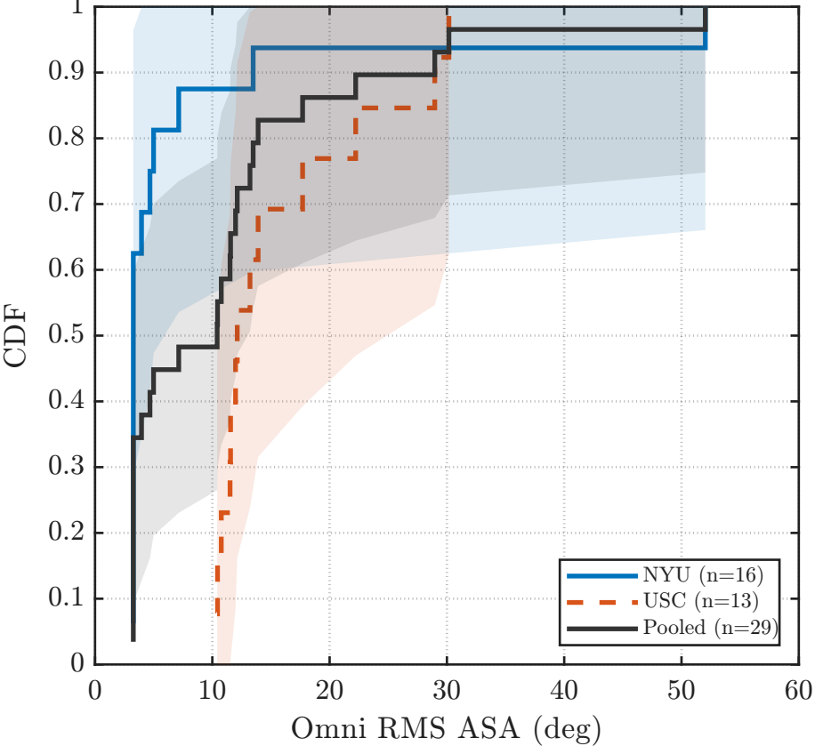
Omni RMS ASA CDF (LOS) - Sub-THz (142 / 145.5 GHz)
