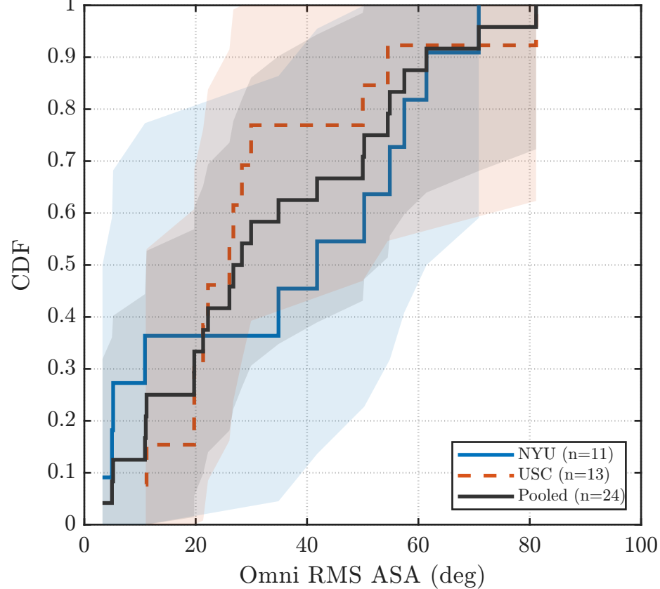
Omni RMS ASA CDF (NLOS) - Sub-THz (142 / 145.5 GHz)
