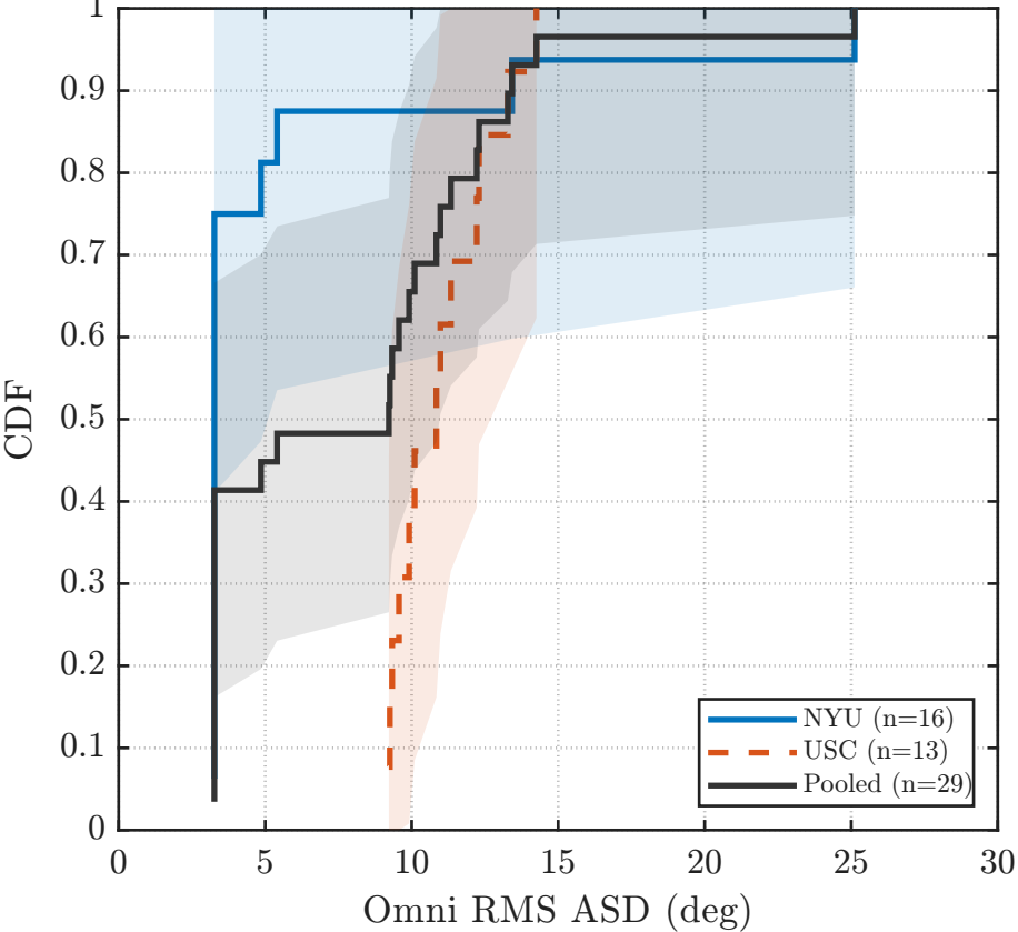
Omni RMS ASD CDF (LOS) - Sub-THz (142 / 145.5 GHz)
