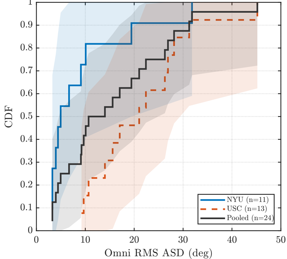
Omni RMS ASD CDF (NLOS) - Sub-THz (142 / 145.5 GHz)
