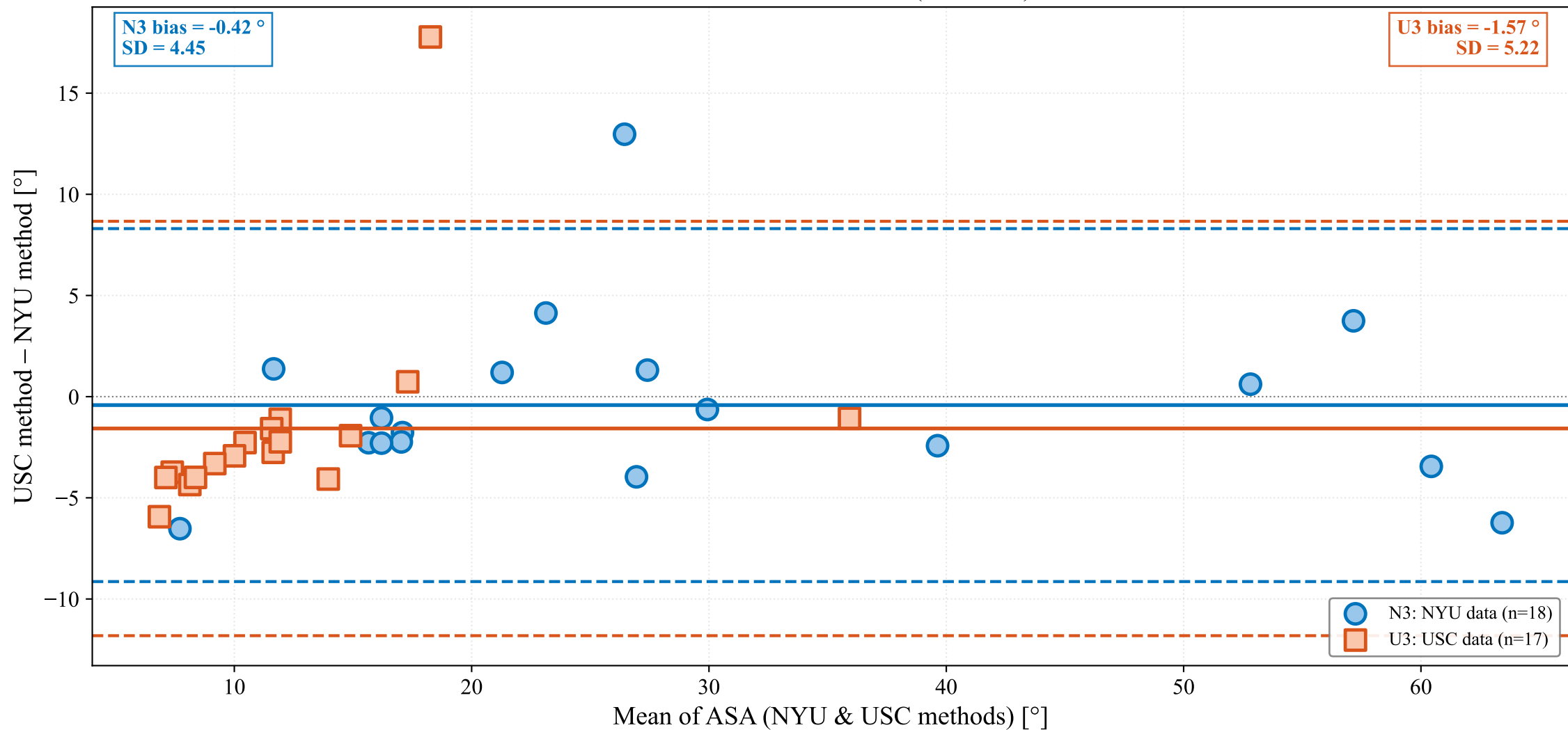
Bland-Altman: Omni ASA (6.75 GHz)
