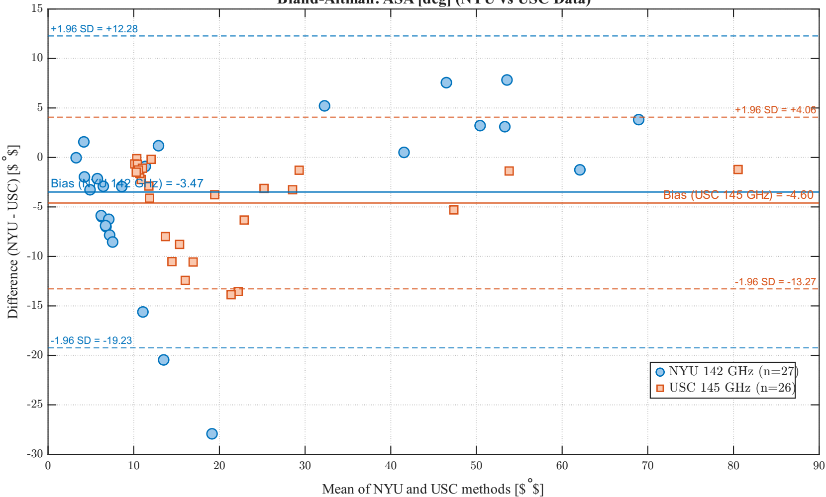
Bland-Altman: ASA [deg] (NYU vs USC Data)
