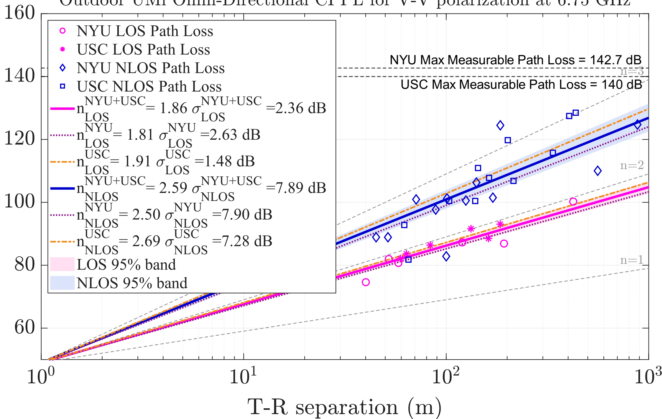
Outdoor UMi Omni-Directional CI PL for V-V polarization at 6.75 GHz
