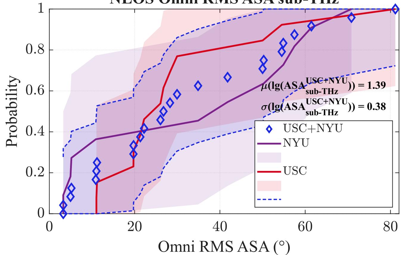
NLOS Omni RMS ASA sub-THz
