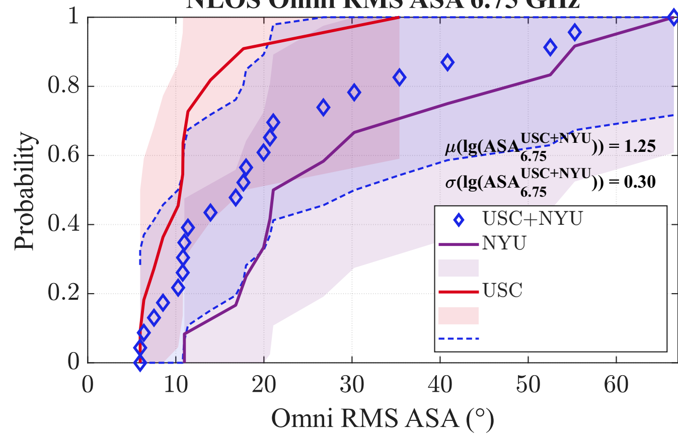
NLOS Omni RMS ASA 6.75 GHz
