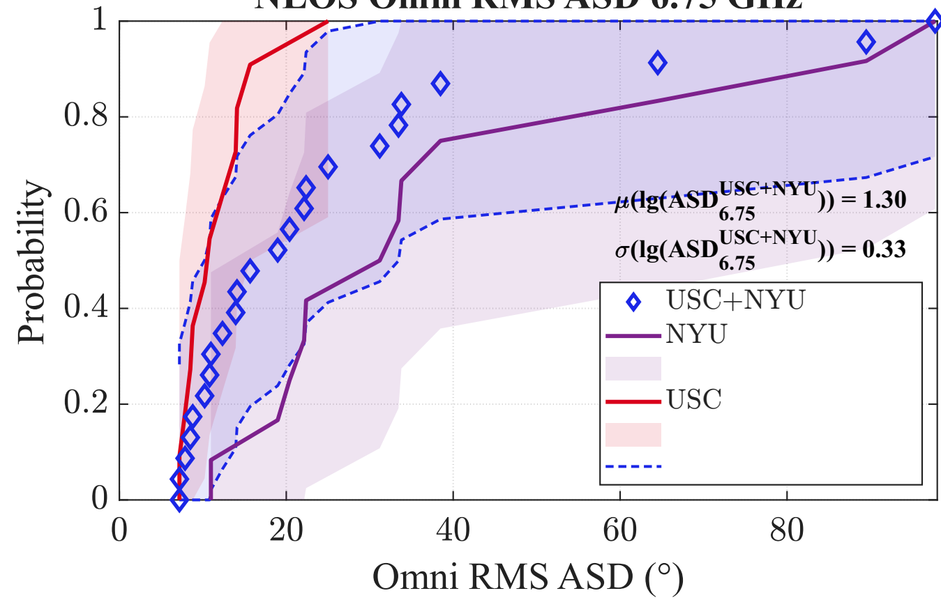
NLOS Omni RMS ASD 6.75 GHz
