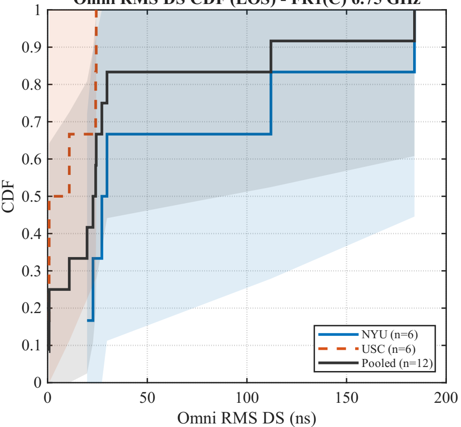
Omni RMS DS CDF (LOS) - FR1(C) 6.75 GHz
