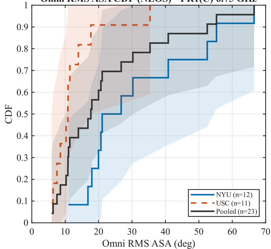
Omni RMS ASA CDF (NLOS) - FR1(C) 6.75 GHz
