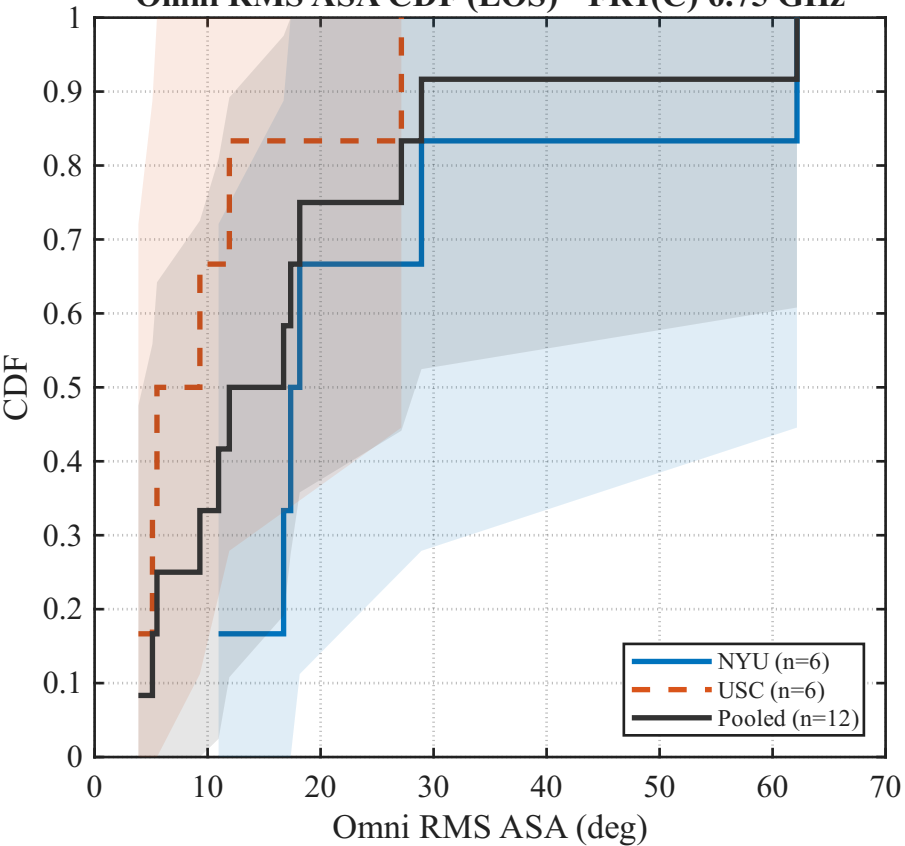
Omni RMS ASA CDF (LOS) - FR1(C) 6.75 GHz
