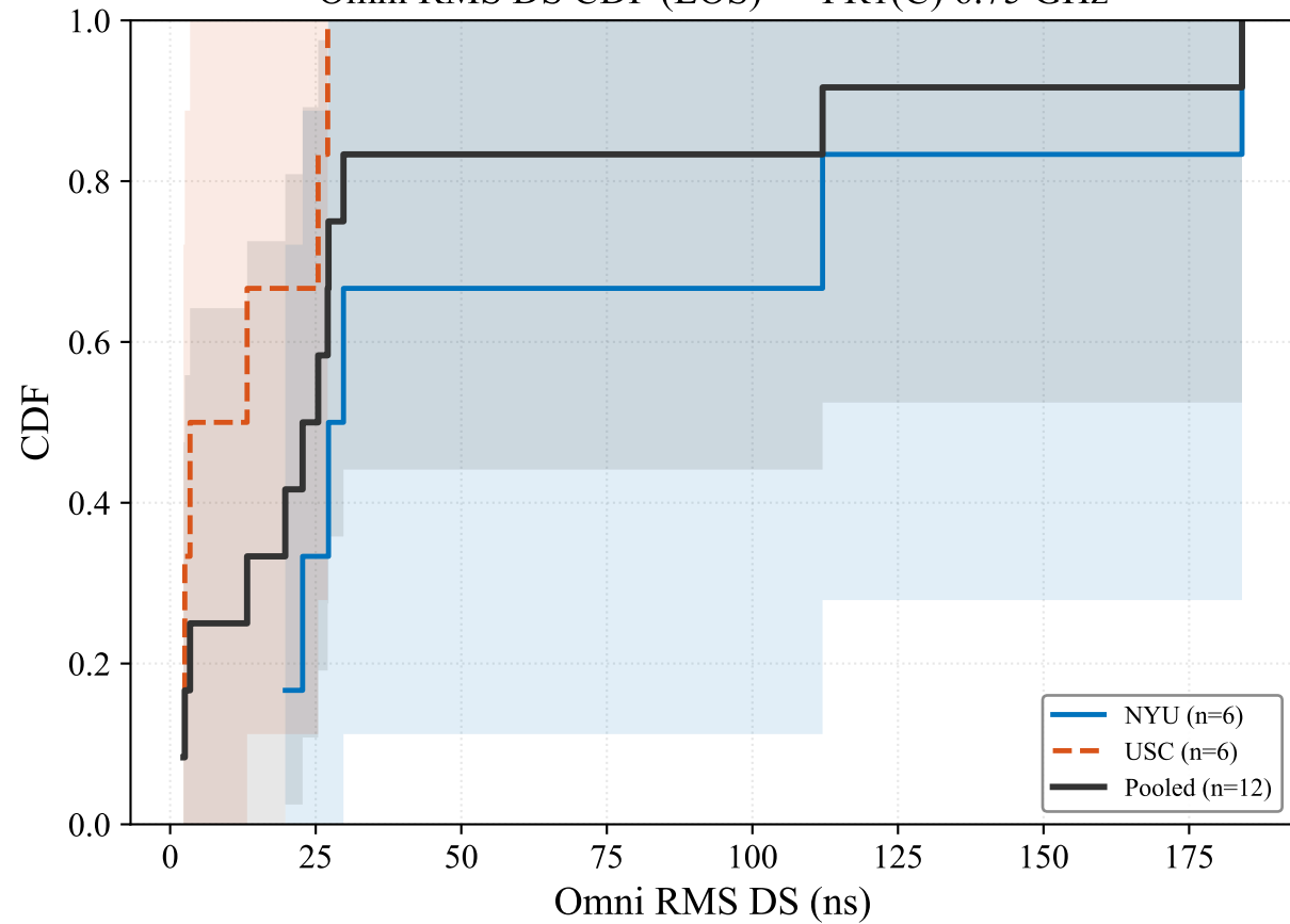
Omni RMS DS CDF (LOS) — FR1(C) 6.75 GHz
