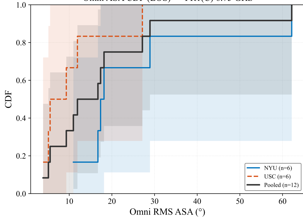
Omni ASA CDF (LOS) — FR1(C) 6.75 GHz
