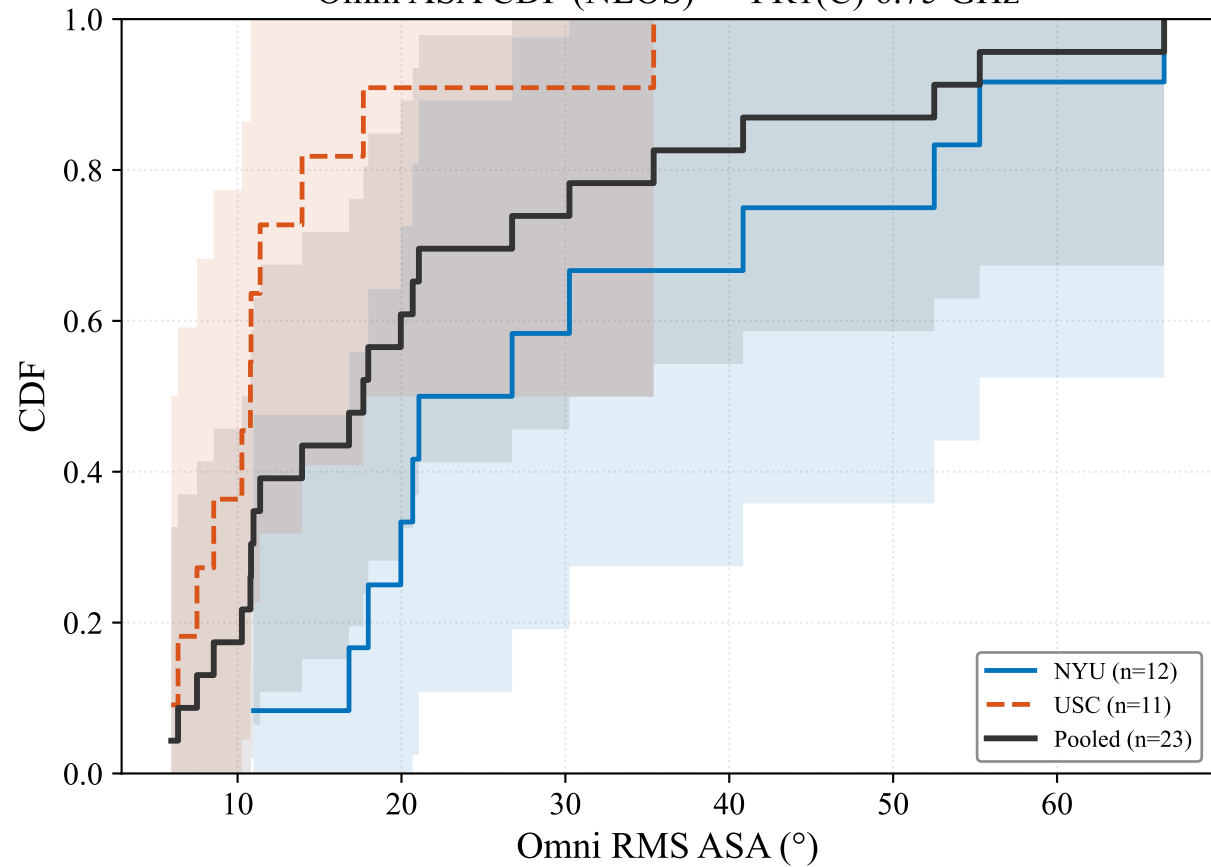
Omni ASA CDF (NLOS) — FR1(C) 6.75 GHz
