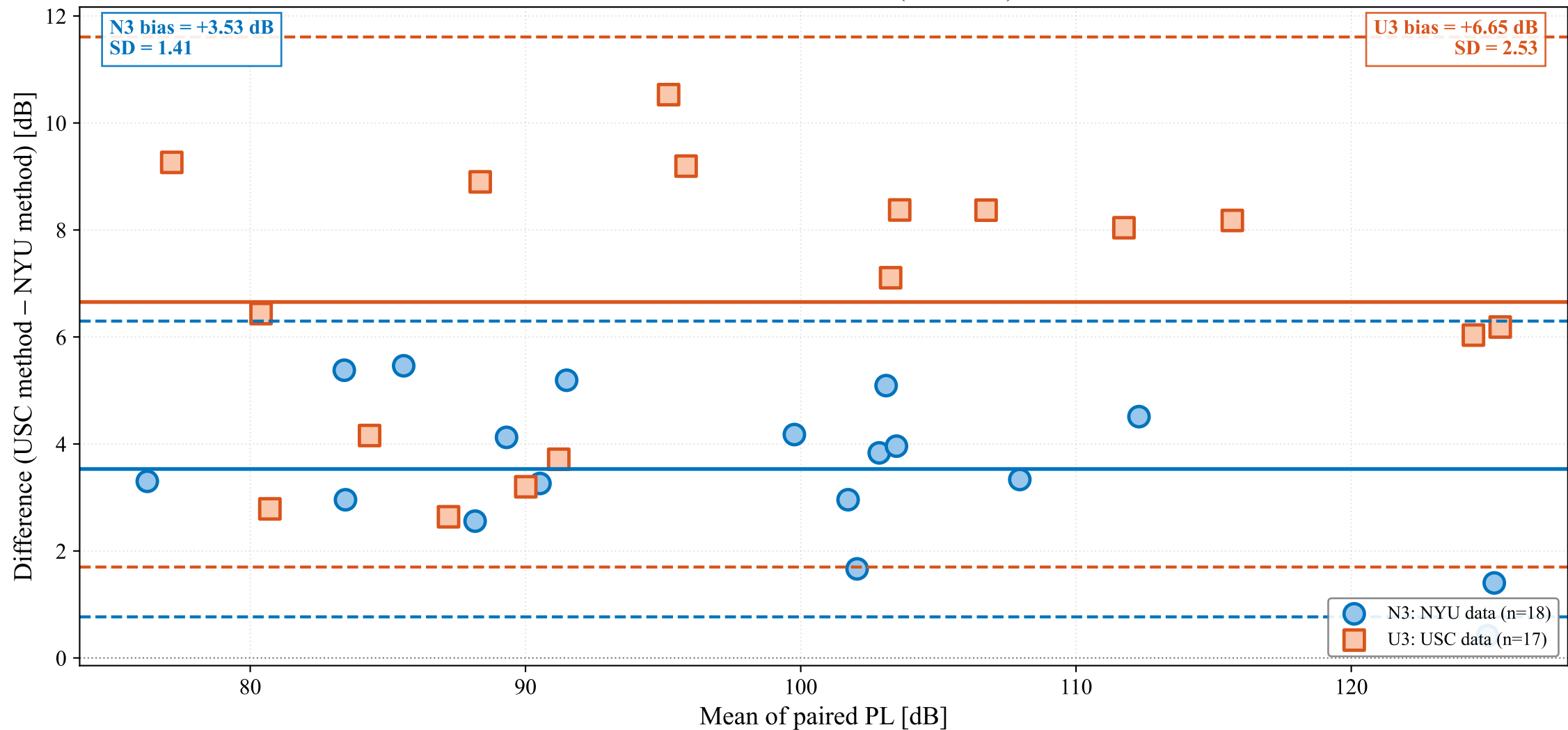
Bland-Altman: Omni PL (6.75 GHz)
