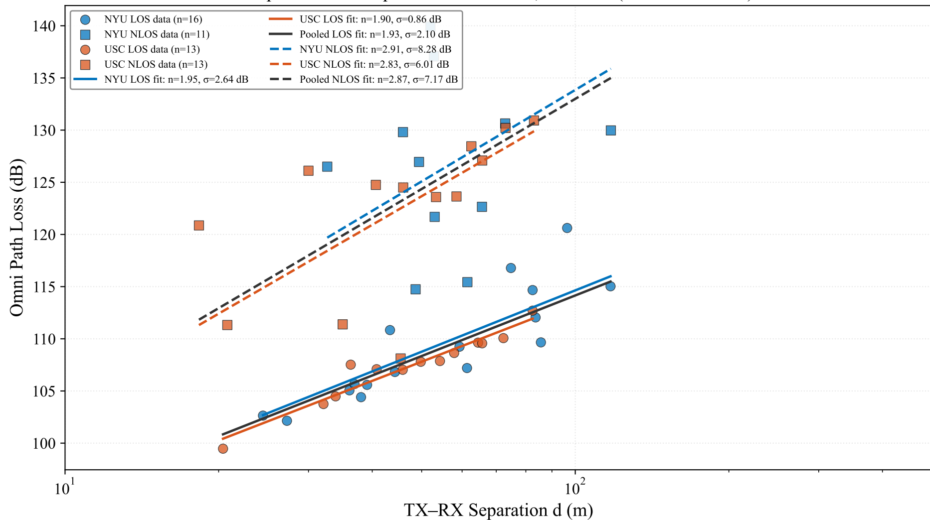
CI path-loss fit — pooled NYU + USC, Sub-THz (142 / 145.5 GHz)
