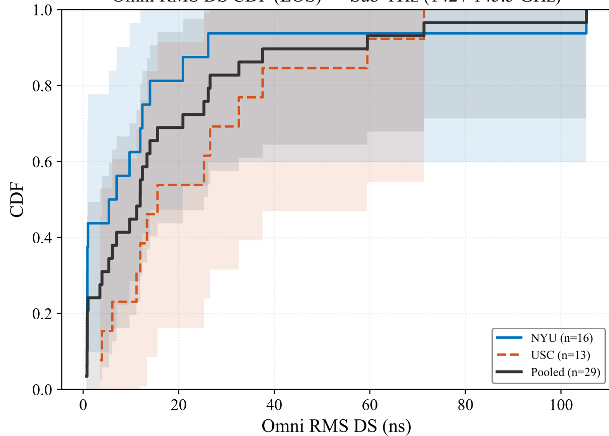
Omni RMS DS CDF (LOS) — Sub-THz (142 / 145.5 GHz)
