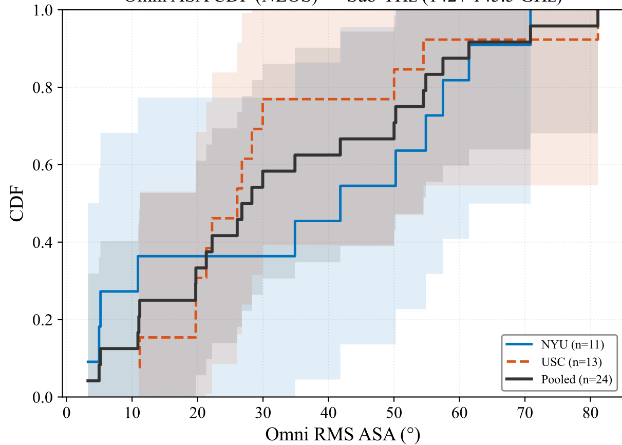
Omni ASA CDF (NLOS) — Sub-THz (142 / 145.5 GHz)
