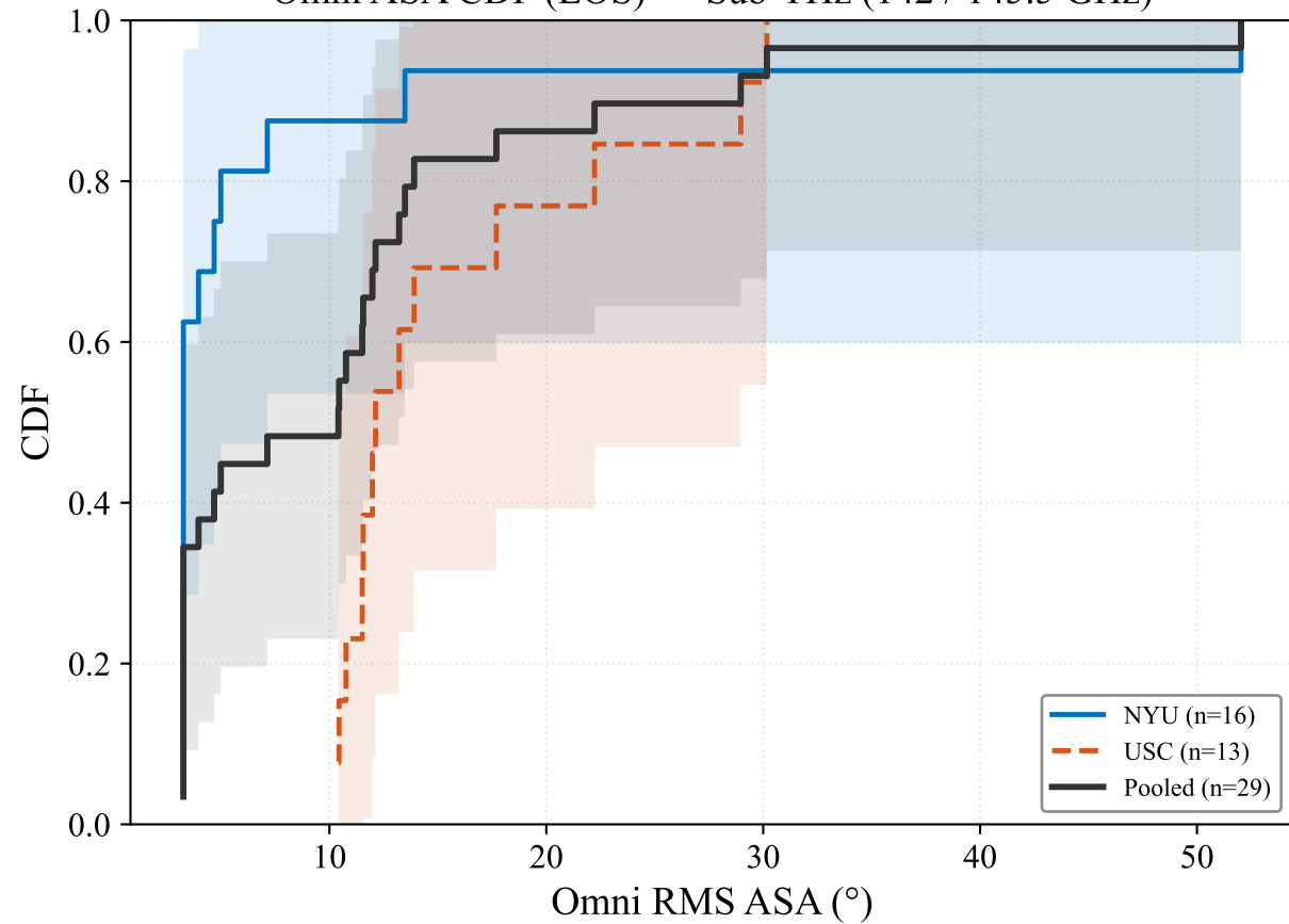
Omni ASA CDF (LOS) — Sub-THz (142 / 145.5 GHz)
