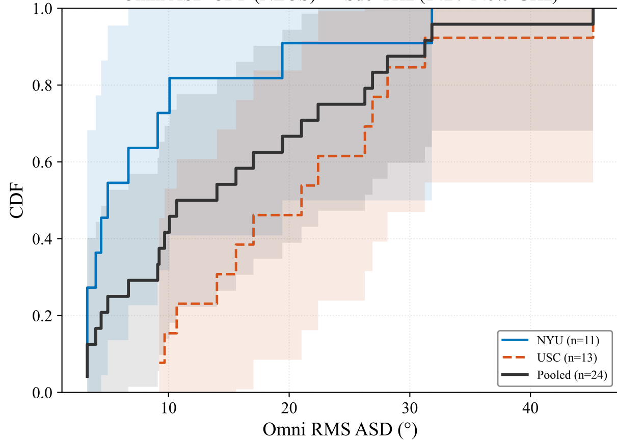
Omni ASD CDF (NLOS) — Sub-THz (142 / 145.5 GHz)
