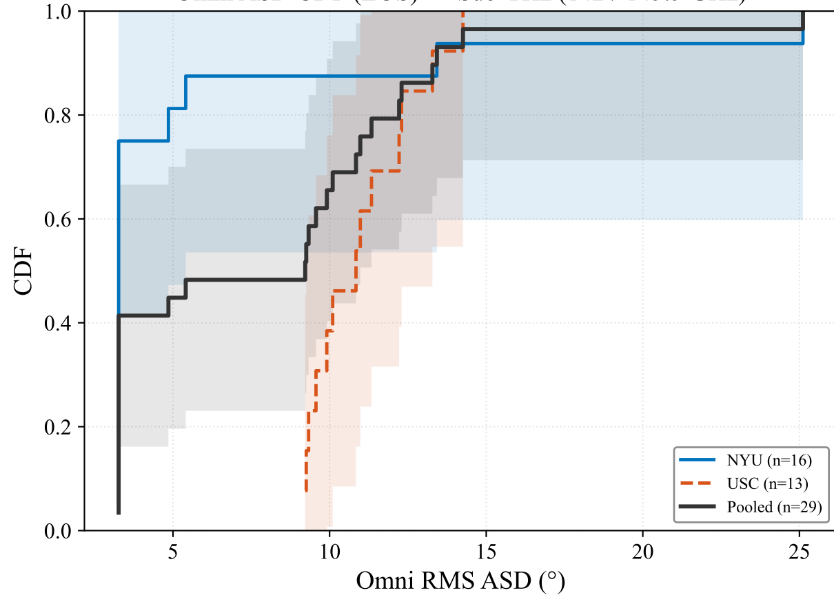
Omni ASD CDF (LOS) — Sub-THz (142 / 145.5 GHz)
