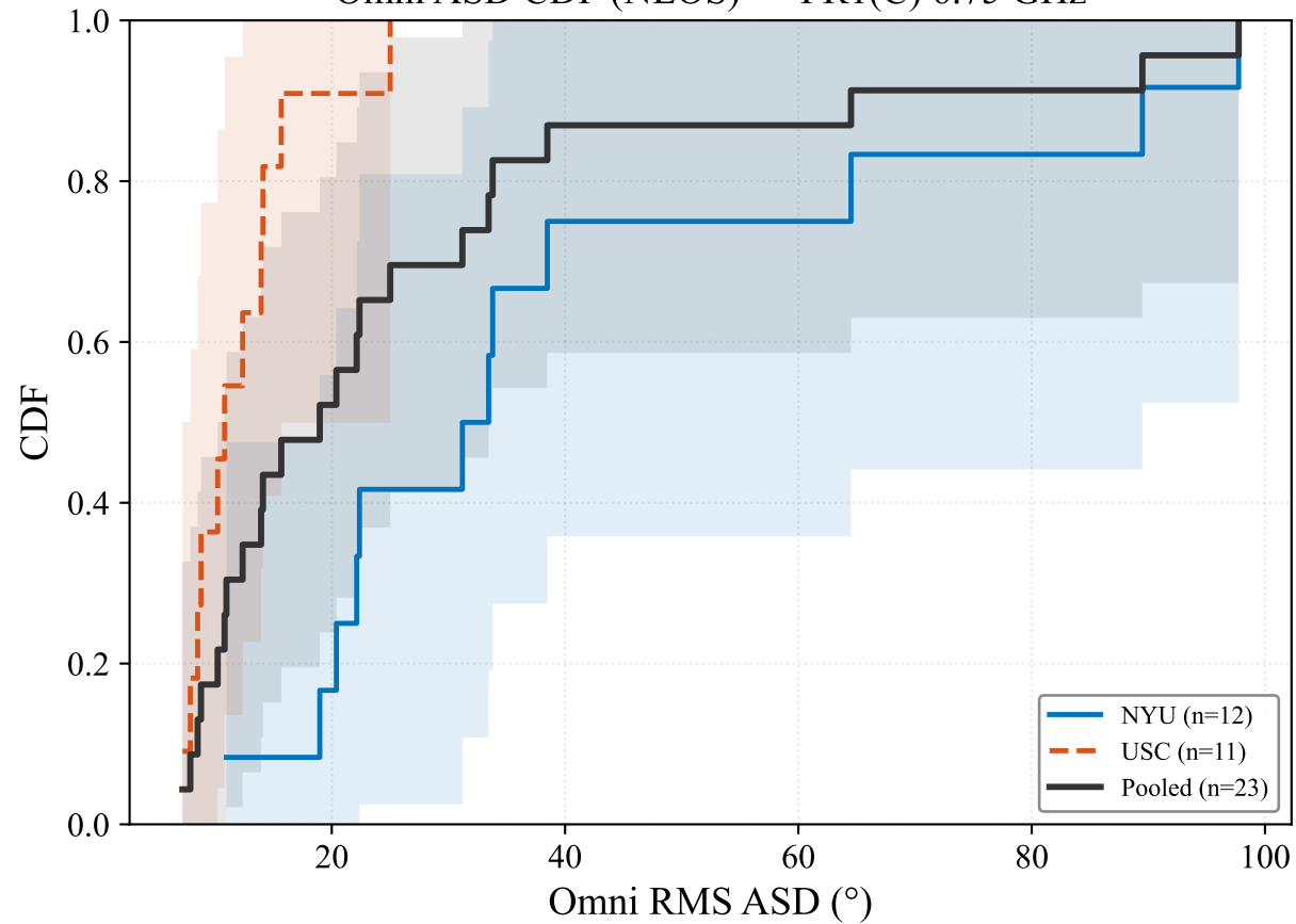
Omni ASD CDF (NLOS) — FR1(C) 6.75 GHz
