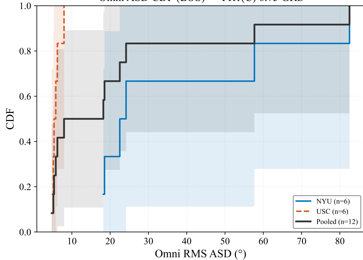
Omni ASD CDF (LOS) — FR1(C) 6.75 GHz
