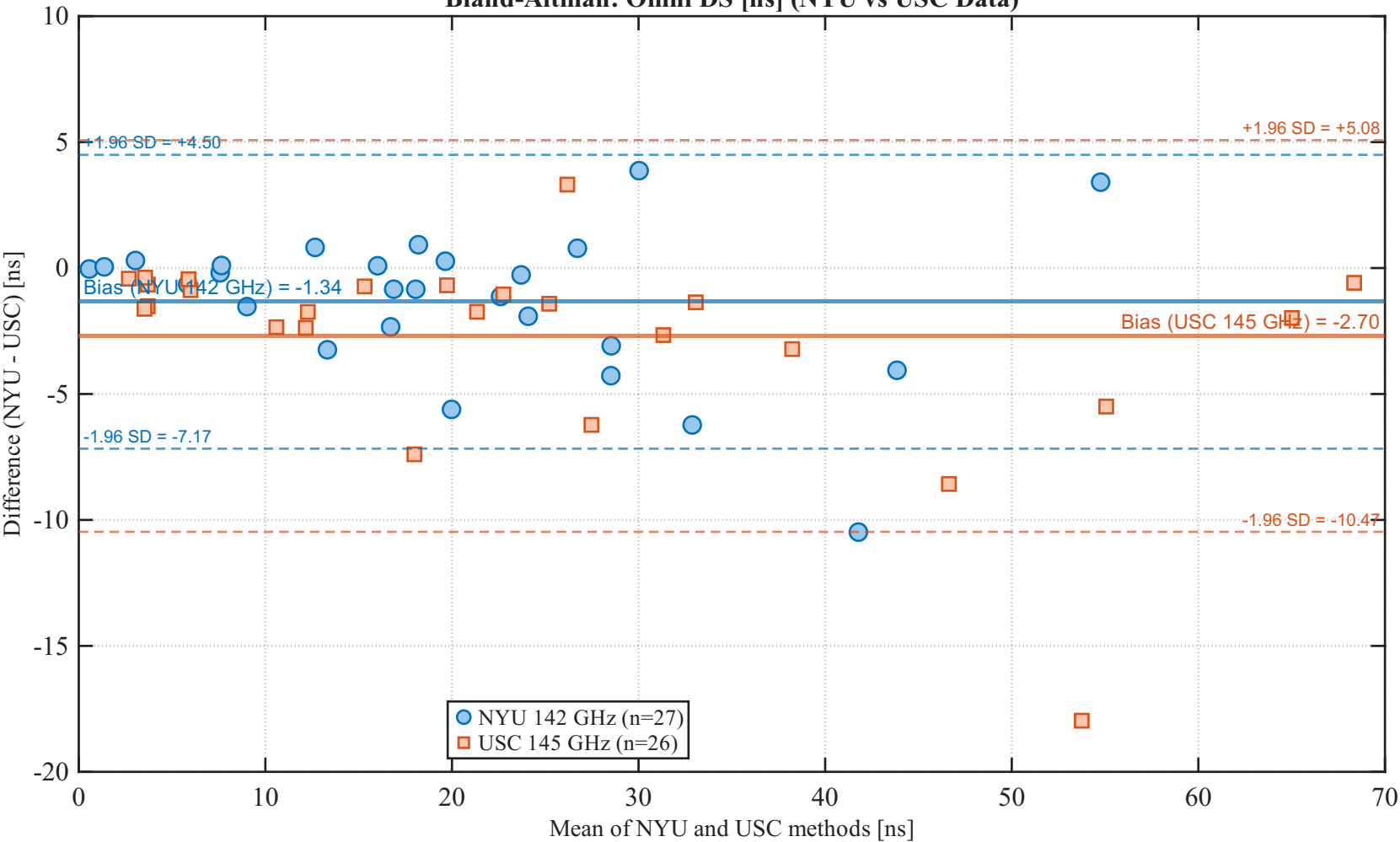
Bland-Altman: Omni DS [ns] (NYU vs USC Data)
