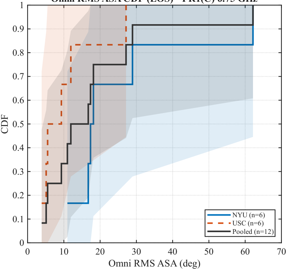
Omni RMS ASA CDF (LOS) - FR1(C) 6.75 GHz
