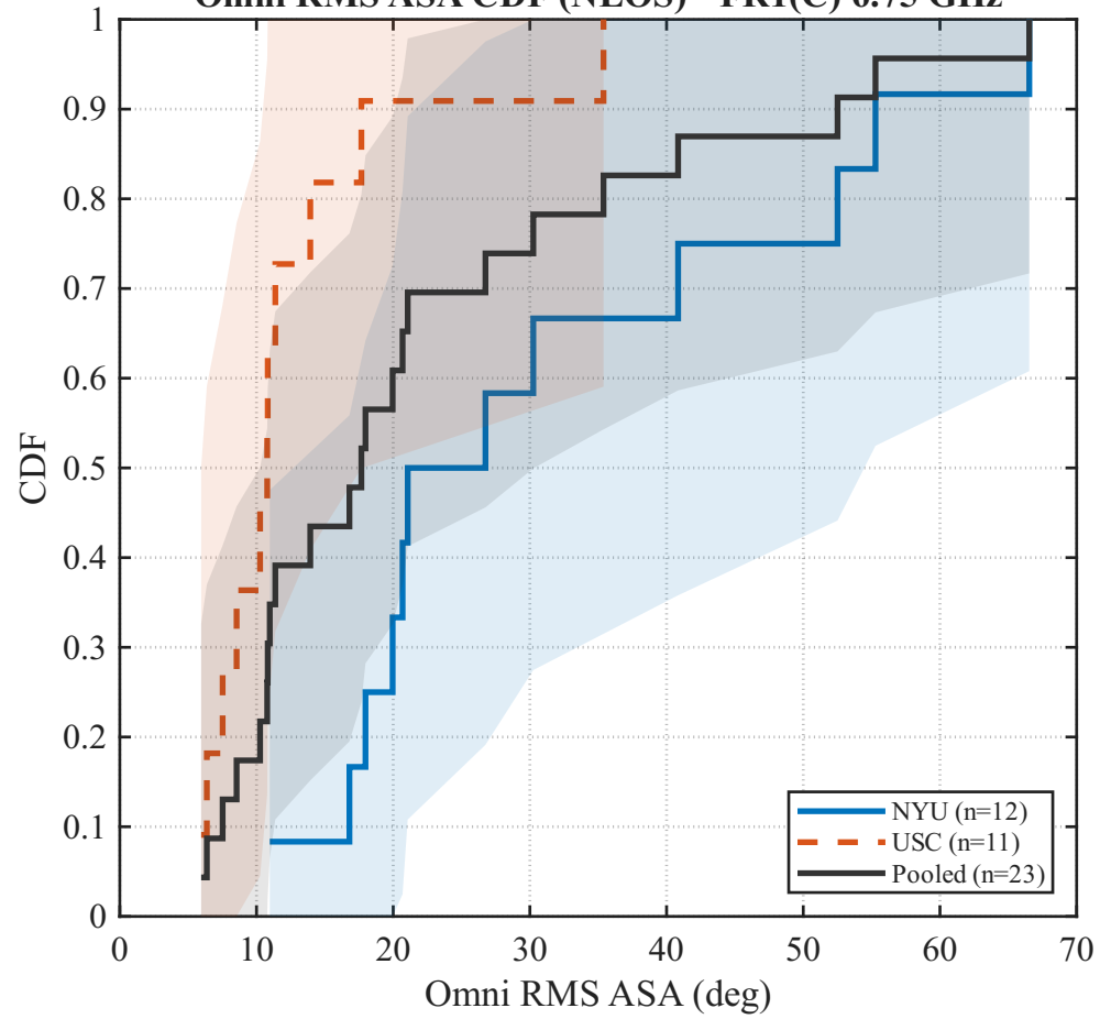
Omni RMS ASA CDF (NLOS) - FR1(C) 6.75 GHz
