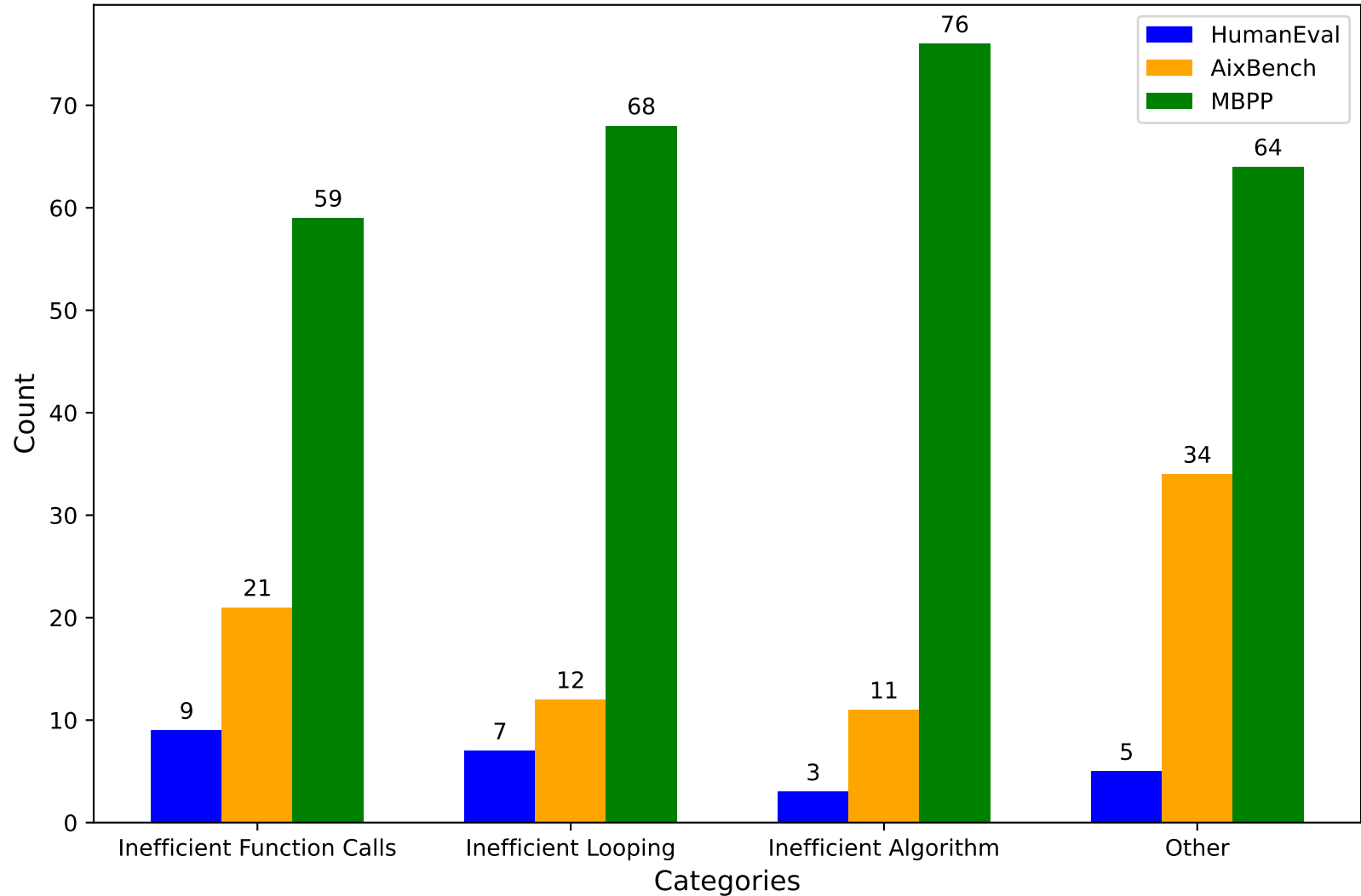
Categories of Patterns Lead to Performance Regression
