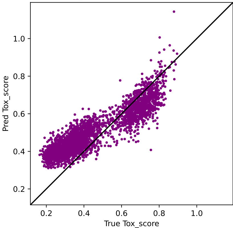
Tox_score (Pearson r = 0.907 )
