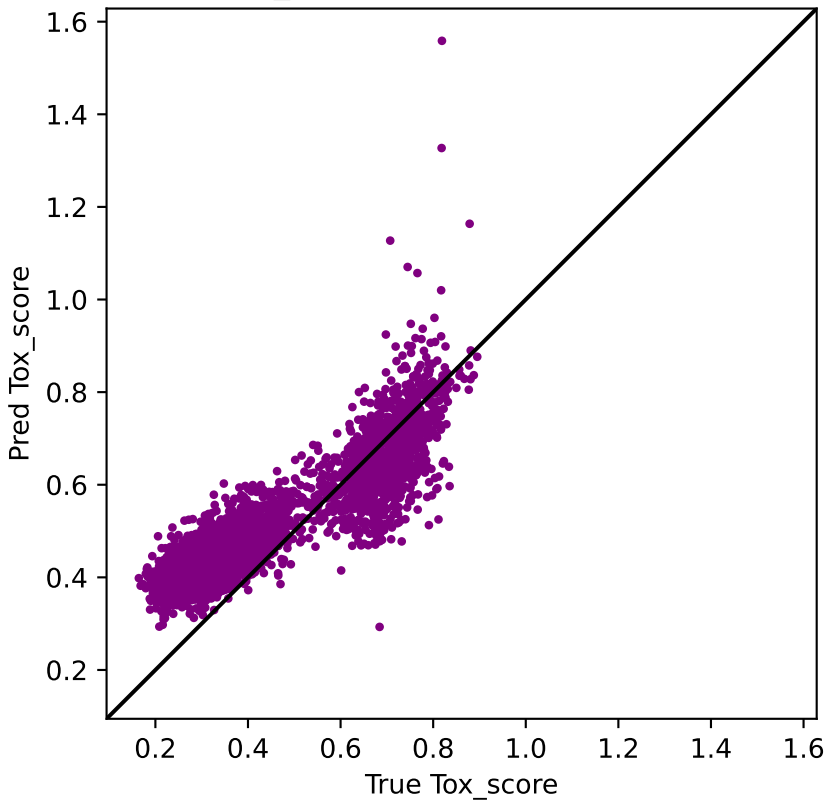
Tox_score (Pearson r = 0.883 )
