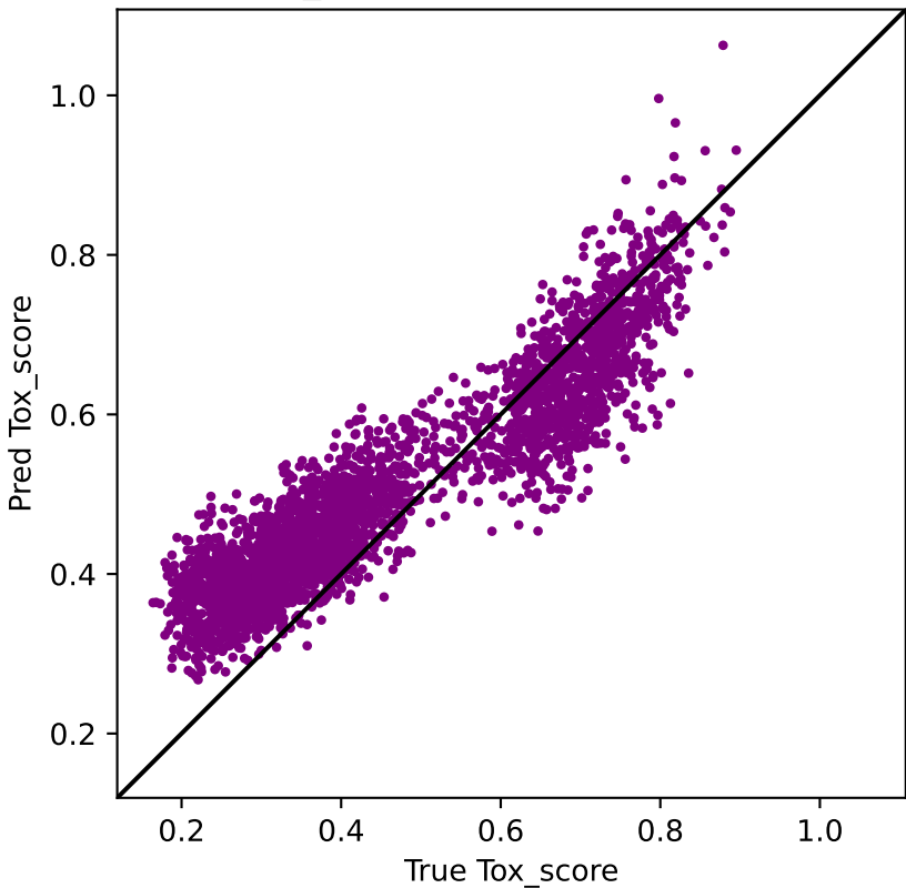
Tox_score (Pearson r = 0.926 )
