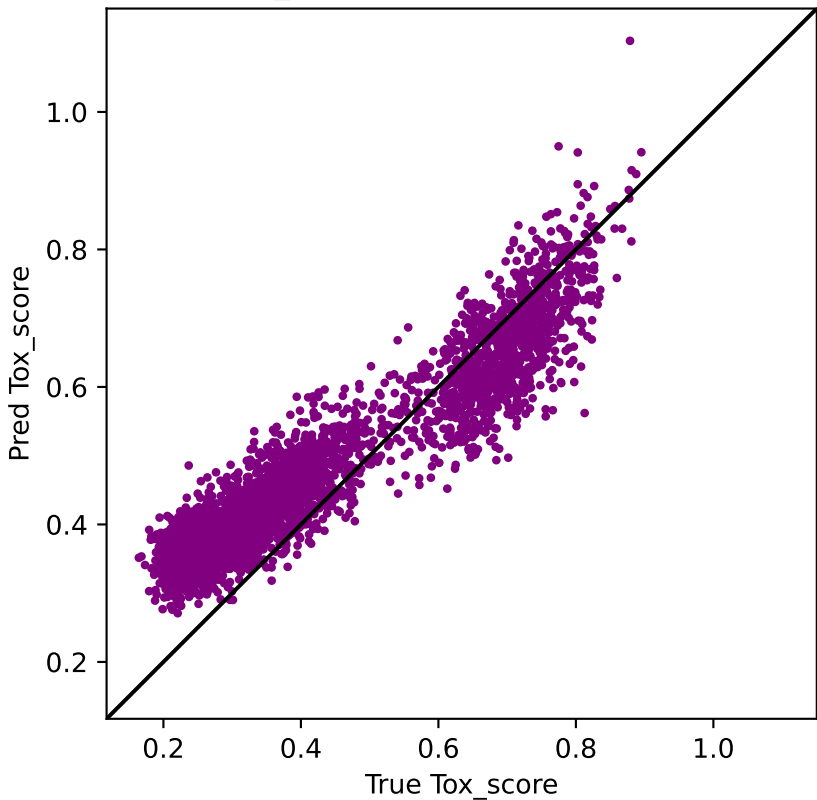
Tox_score (Pearson r = 0.939 )
