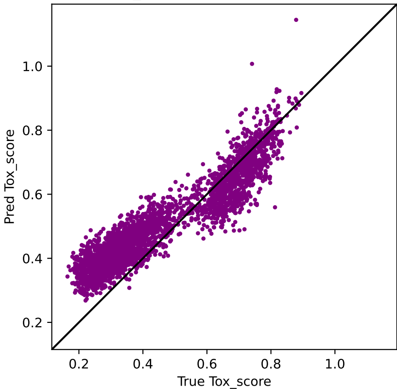
Tox_score (Pearson r = 0.931 )
