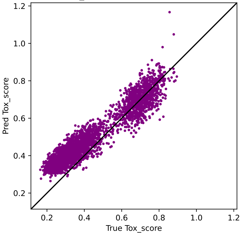
Tox_score (Pearson r = 0.951 )
