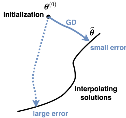
Figure 4: The original informal sketch of algorithmic solution selection. For the linear problem here, the set of exact fits is affine, rather than the curved set in the sketch. Zero initialization and the update rule select the nearest exact fit to the origin. Original course asset; its external provenance is not specified in the original notes.
