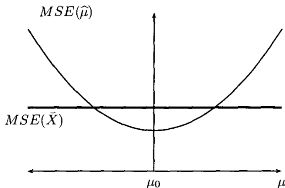
Figure 1: The original risk sketch: shrinkage wins near the reference \mu_0 and loses far away. The horizontal axis varies the unknown true mean, not the observed sample. Retained from the original notes, which attribute the figure to [3].
