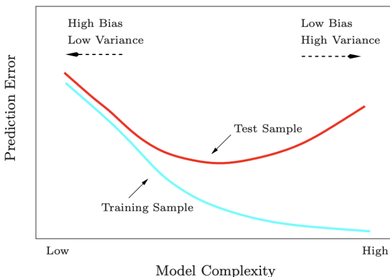
Figure 2: The classical picture: greater flexibility can reduce squared bias while increasing variance, producing a useful middle ground for prediction. This is a schematic pattern, not a universal shape for every risk curve. Figure retained from the original notes, attributed there to [4].
