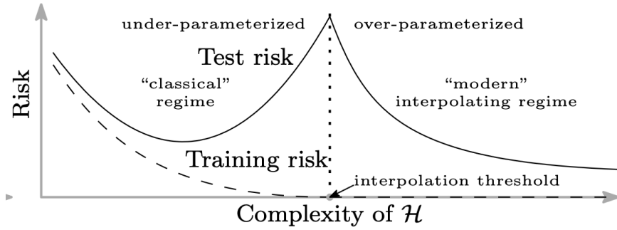
Figure 3: A schematic second descent beyond the interpolation threshold. Retained from the original notes, attributed there to [2]. It summarizes a possible risk pattern; the preceding bounds require explicit spectral assumptions.
