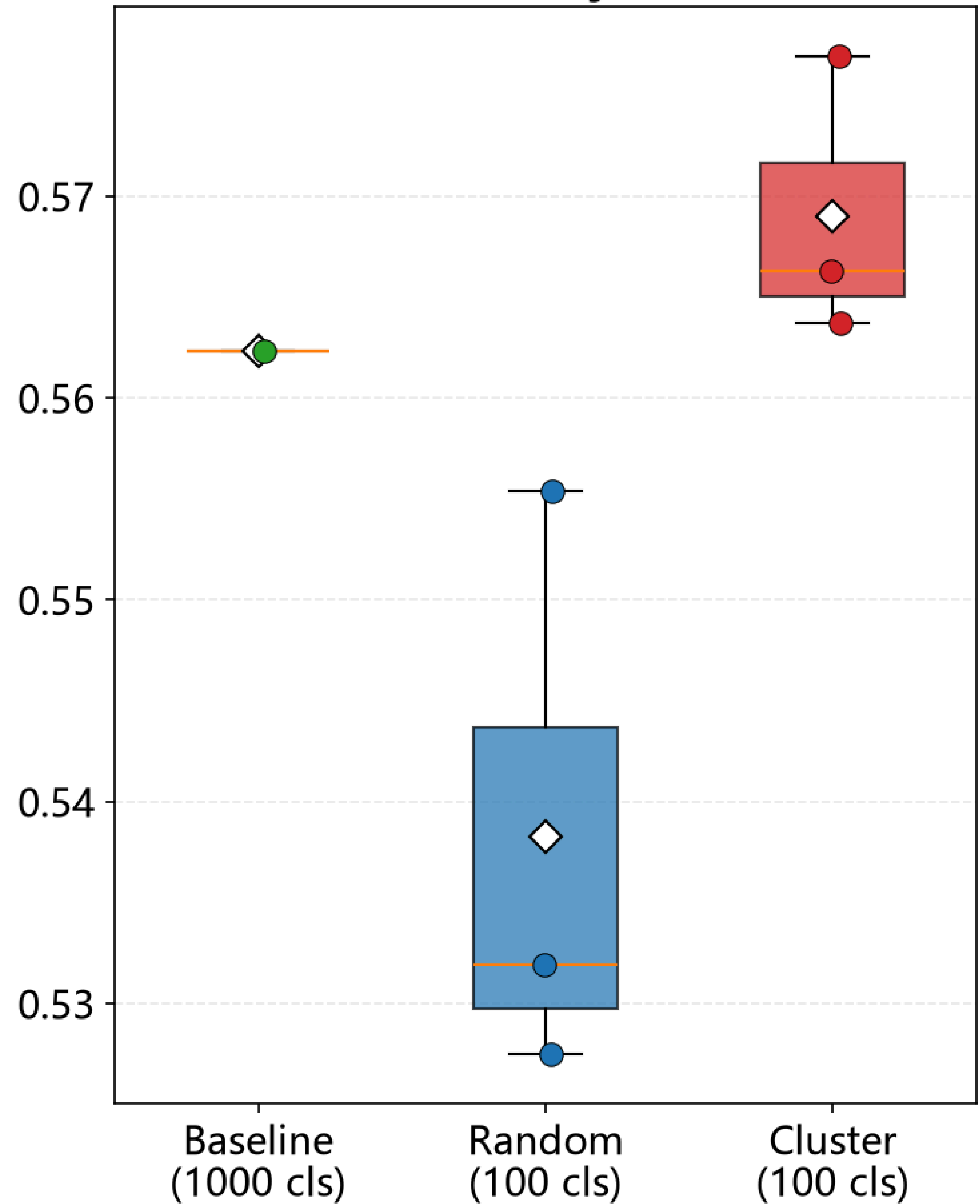
Authenticity Norm
