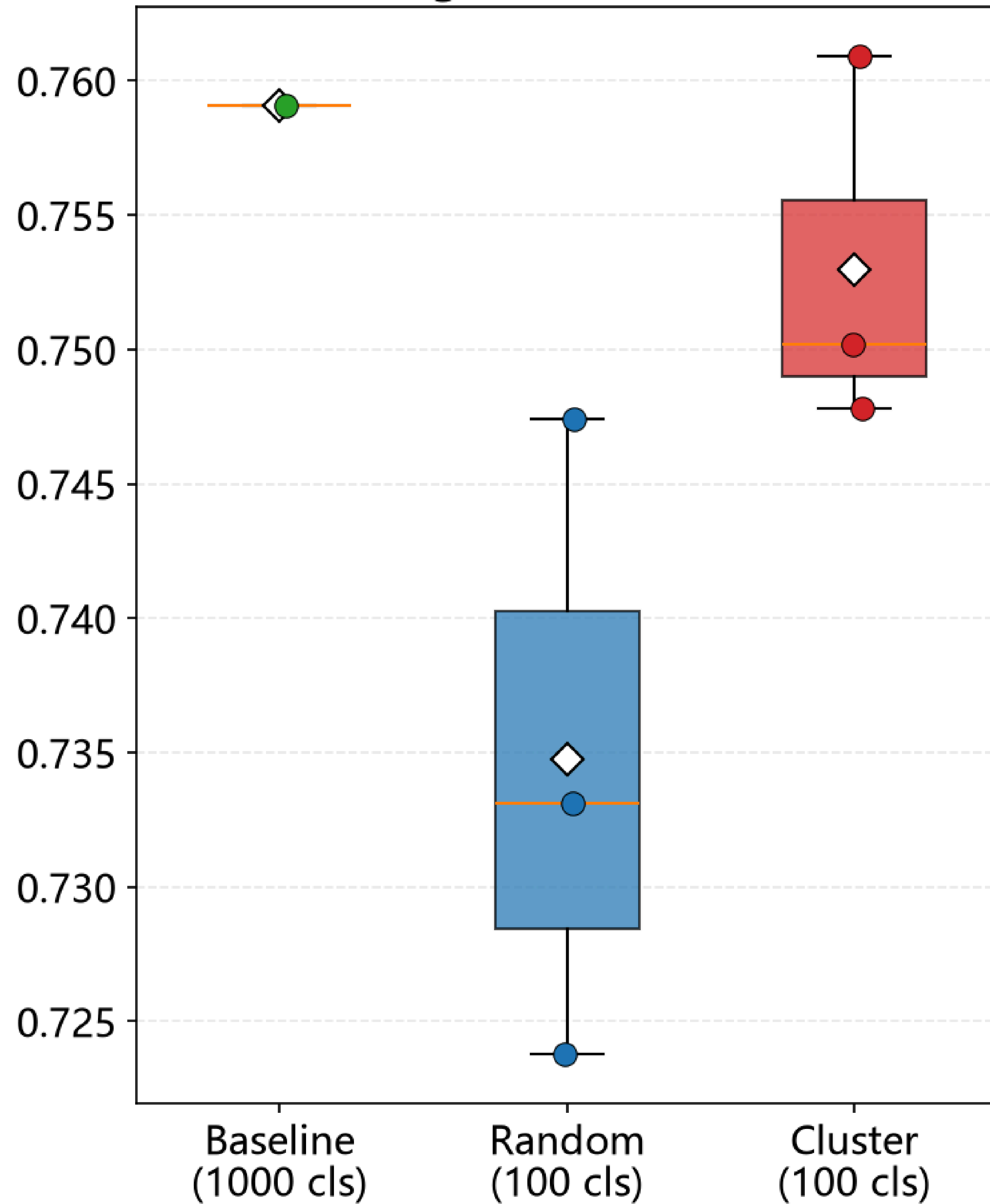
Alignment Norm
