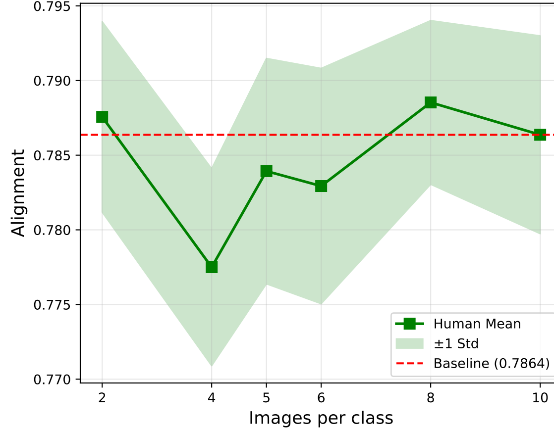
(b) Human Stability - Alignment
