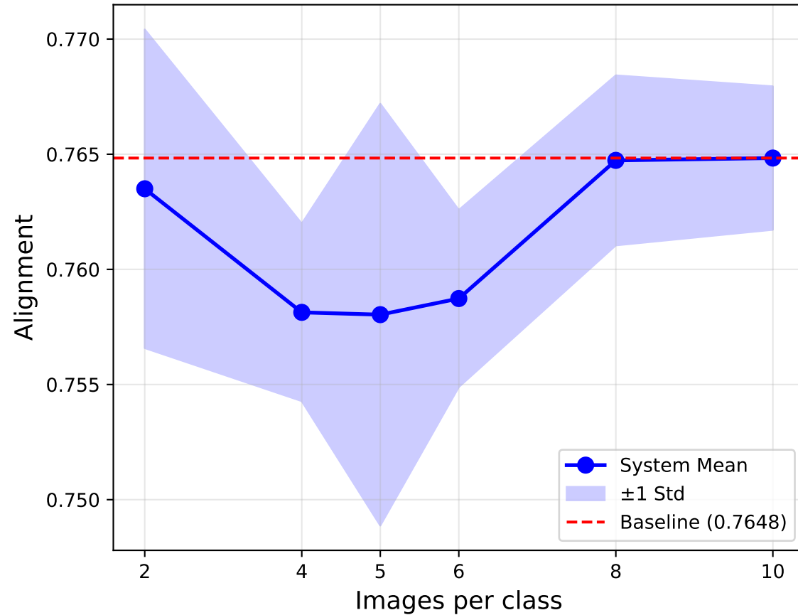
(a) System Stability - Alignment
