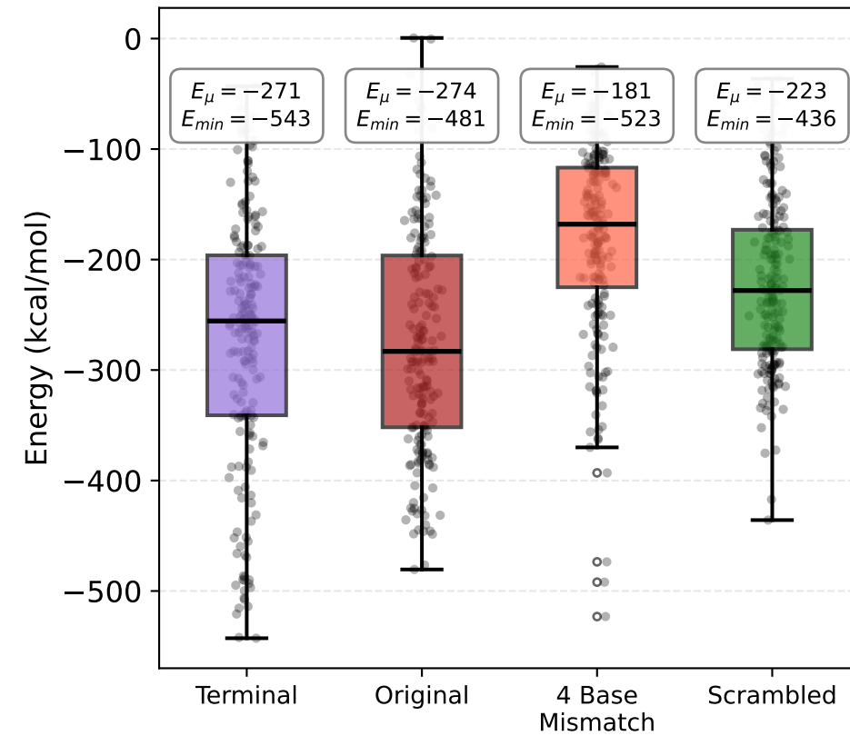
Total Energy (Sum of All 3)
