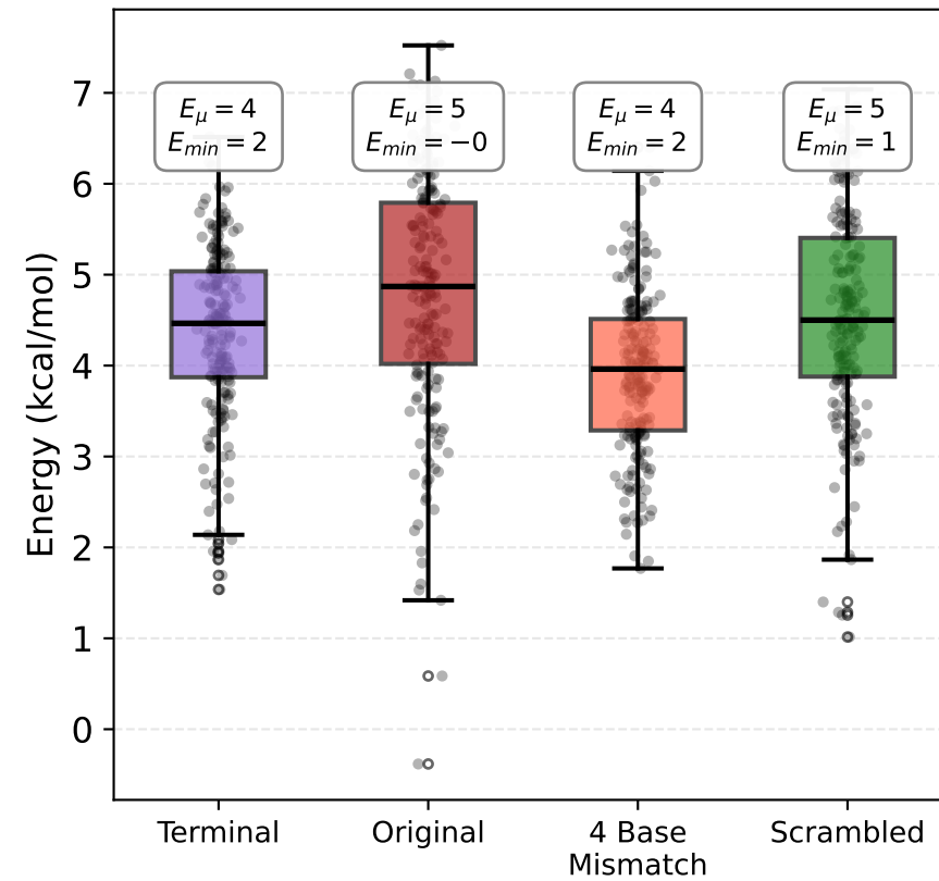
Desolvation Energy
