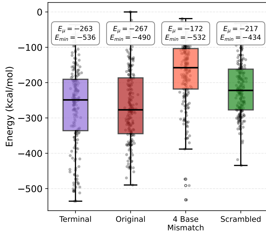
Electrostatic Energy
