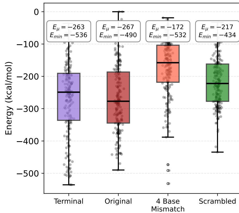
Electrostatic Energy
