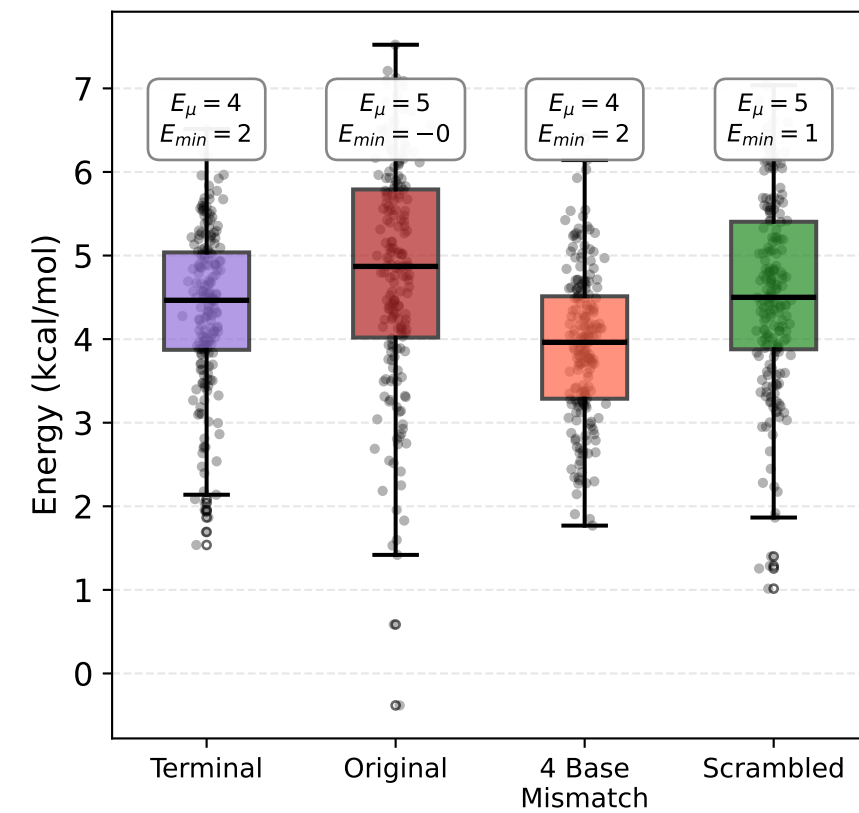
Desolvation Energy
