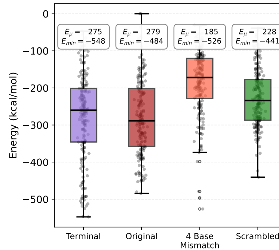
Non-bonded Energy
