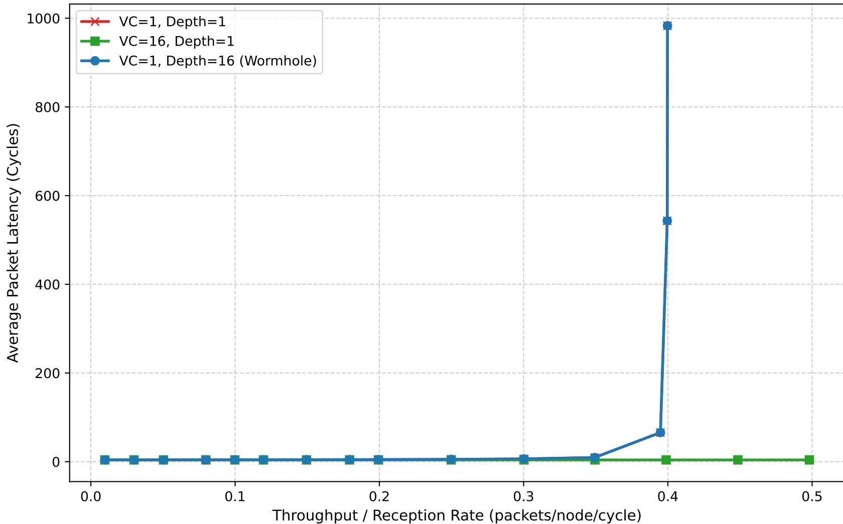
Buffer Allocation Comparison (Tornado, 16-Node 4x4 Mesh)
