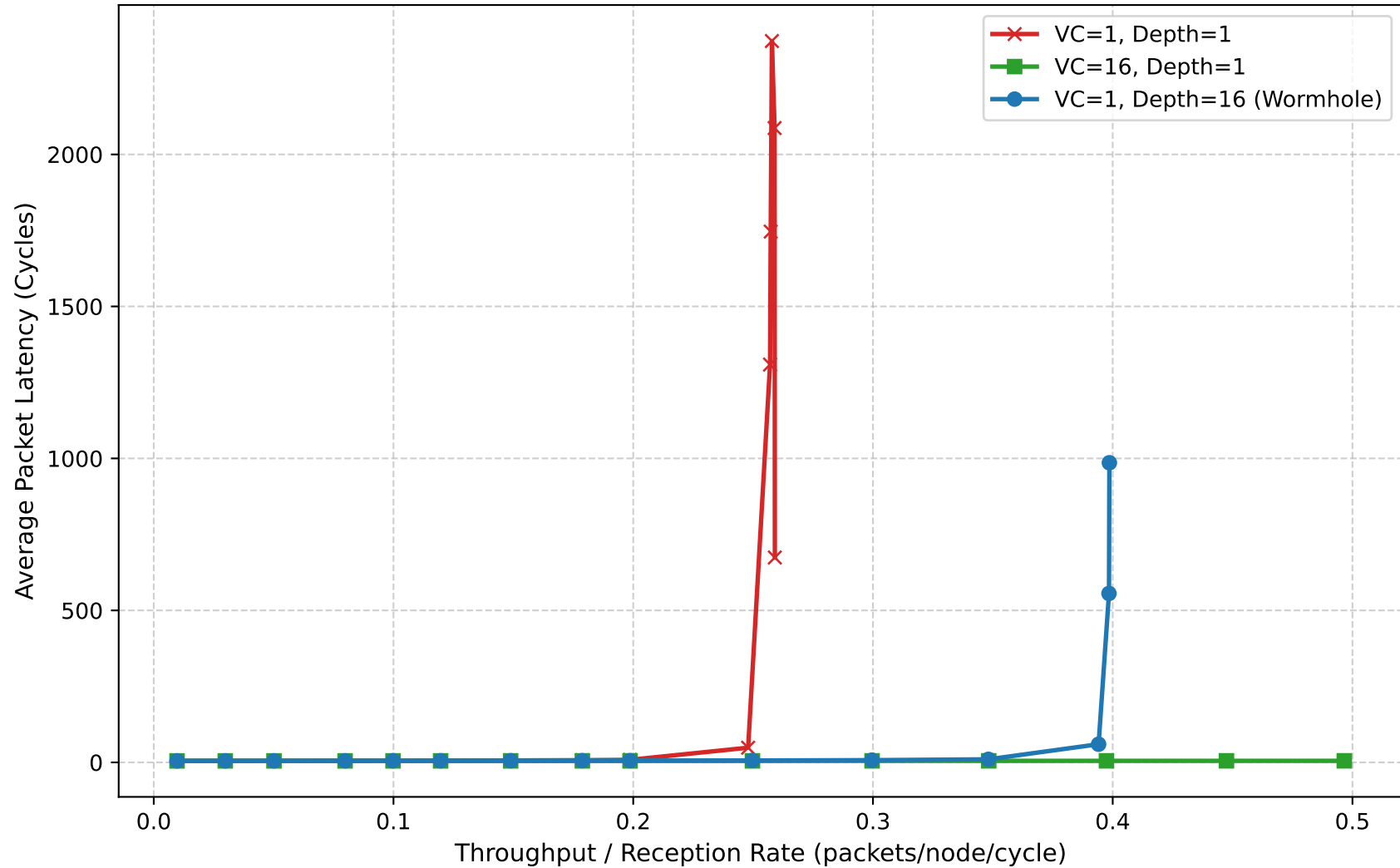
Buffer Allocation Comparison (Uniform Random, 16-Node 4x4 Mesh)
