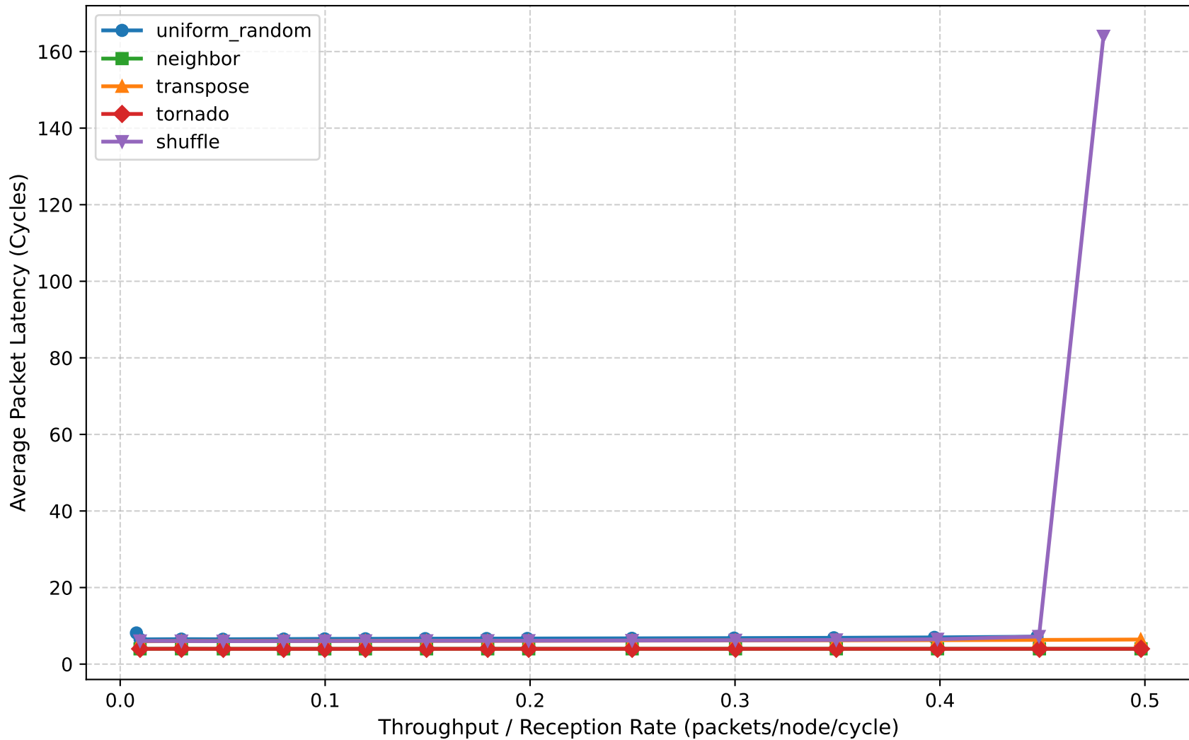
Ring Topology (16 Nodes): Latency vs. Throughput
