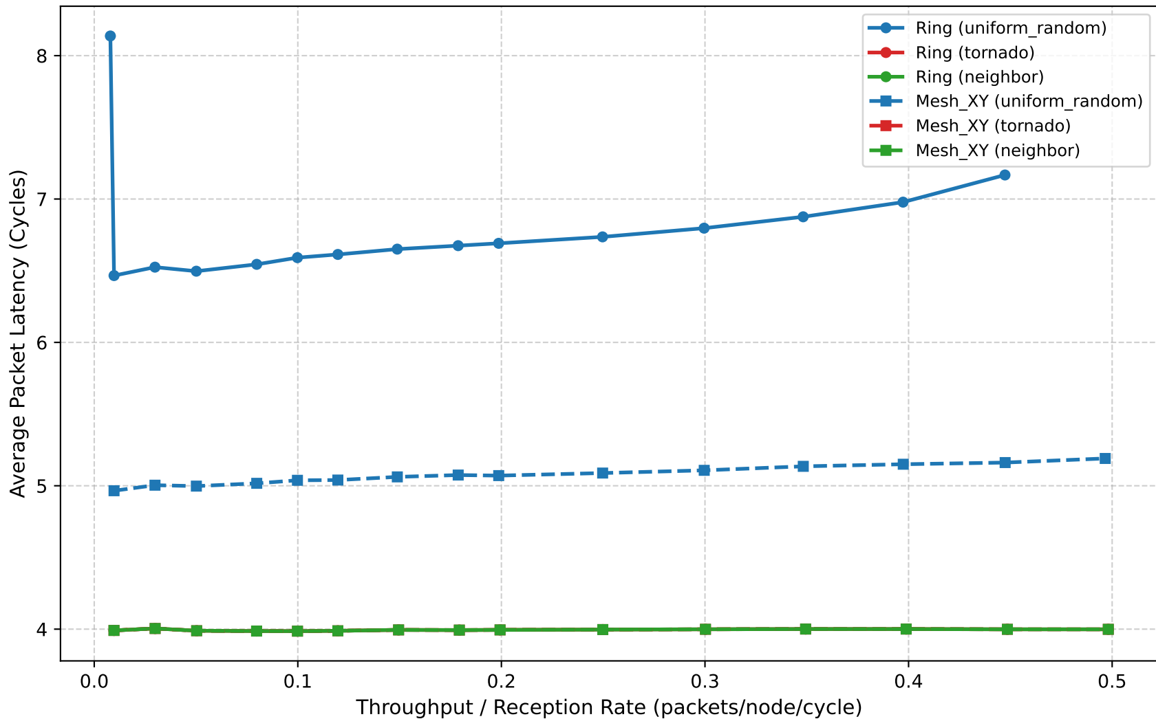
16-Node Comparison: Ring (1D-Torus) vs. 4x4 Mesh
